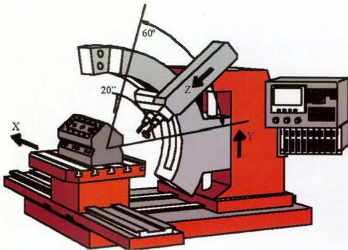
Figure 3: Arch-Type Machining
