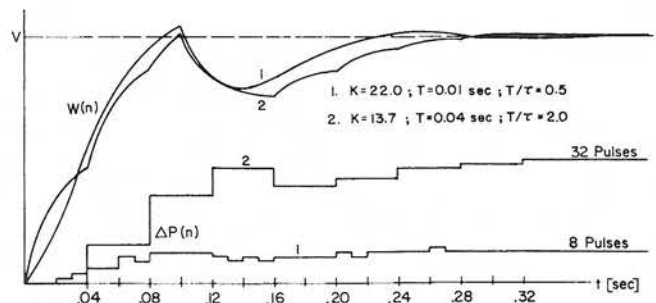
Fig. 7 Responses and counter readings of a simulated Sampled-Data system
