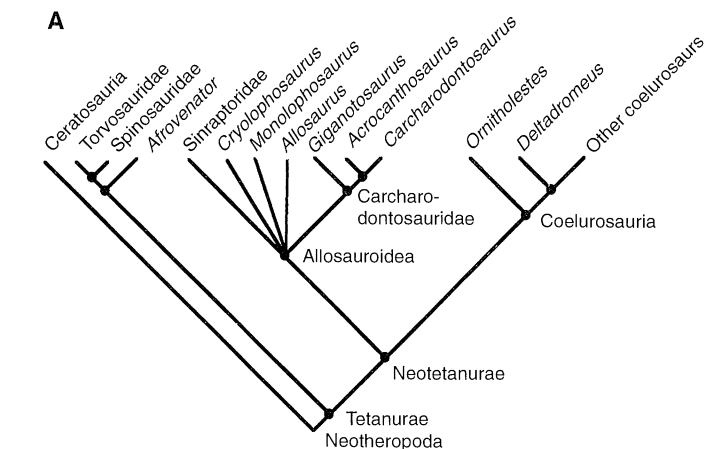
Fig. 4. Phylogenetic and temporal relationships among basal tetanurans.
