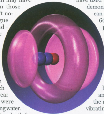
HELIUM BALLOONS Large ring marks where helium atoms first surround a nitrous oxide molecule. Hints of superfluidity start as additional helium atoms occupy hubcap-shaped end regions.
