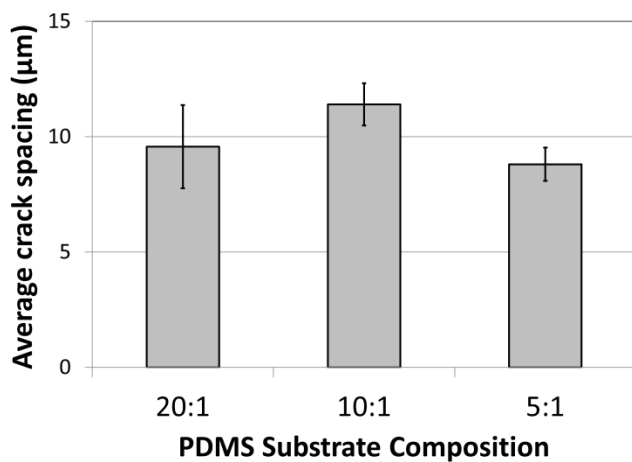
Figure S2. Crack spacing does not vary significantly with PDMS substrate composition. The monomer: crosslinker ratio was modified to change the mechanical properties of the PDMS layer. However, no
