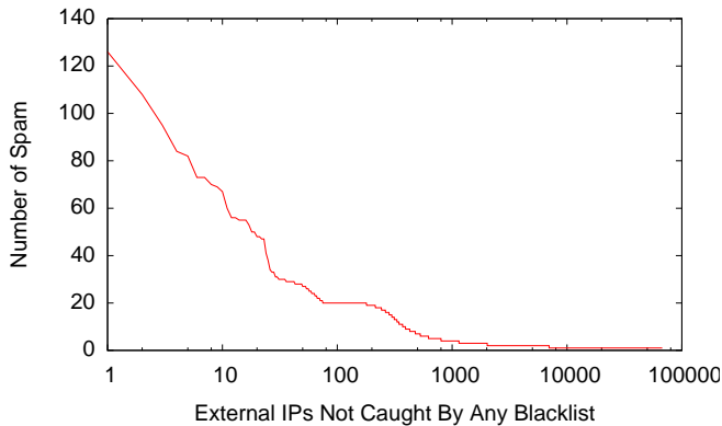
Figure 5. Spam missed by blacklists (false negatives) binned by source IPs external to the network. Most sources sent very few spams to our network.
