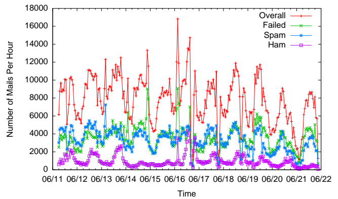
Figure 1. Number of mails per hour observed on the academic network. The overall mail rate is further divided by ham, spam, and failed connections.
