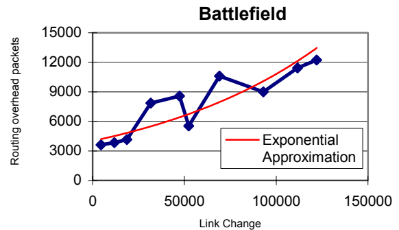
Figure 4. Routing overhead vs link change.
