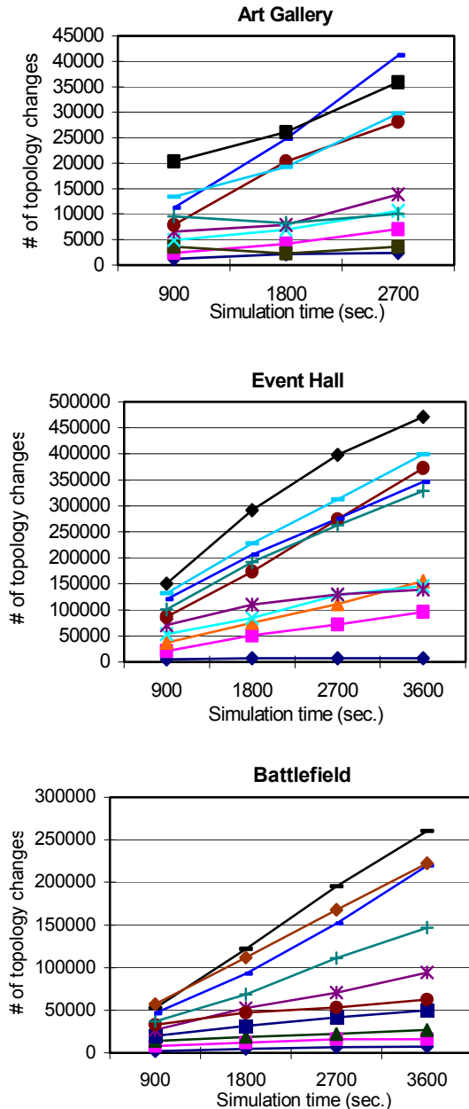
Figure 2. Linear relation between simulation time and number of topology change.
