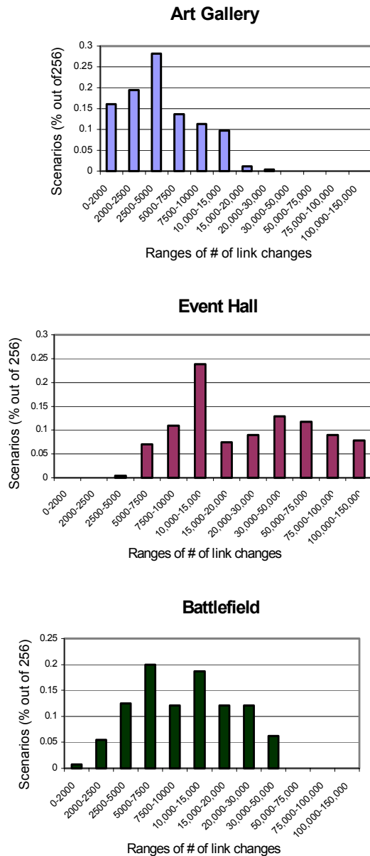
Figure 1. Distribution of number of scenario files according to number of topology changes during 900-second simulation.
