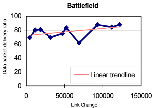
Figure 3. Data packet delivery ratio (%) vs link change.
