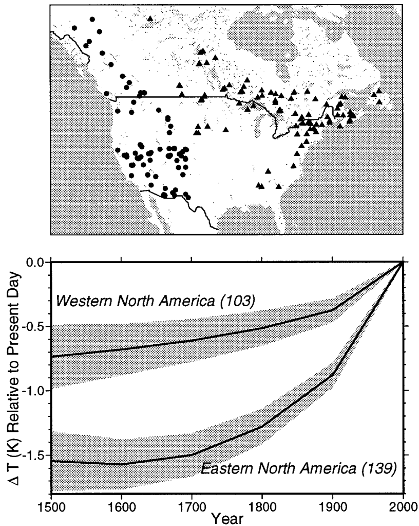
Figure 5 (Top) Map of borehole sites in North America; western sites shown by dots , eastern sites by triangles . (Bottom) Reconstruction of the surface temperature history over the past 5 centuries for western and eastern North America, as determined from borehole temperatures at sites shown at top . Shaded areas represent \pm 1 standard error about the mean histories.
