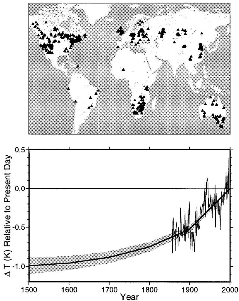
Figure 7 (Top) Map of borehole sites in the global database of borehole temperatures (Huang & Pollack 1998) used in reconstructing a global mean ground surface temperature history. (Bottom) Reconstruction of the surface temperature history inferred from borehole temperatures at sites shown above (Pollack & Huang 1998, Huang et al 2000). Shaded area represents \pm 1 standard error about the mean history. Also shown for comparison is a 5-year running mean of the globally averaged instrumental record of surface air temperature since 1860 (Jones et al 1999a).
