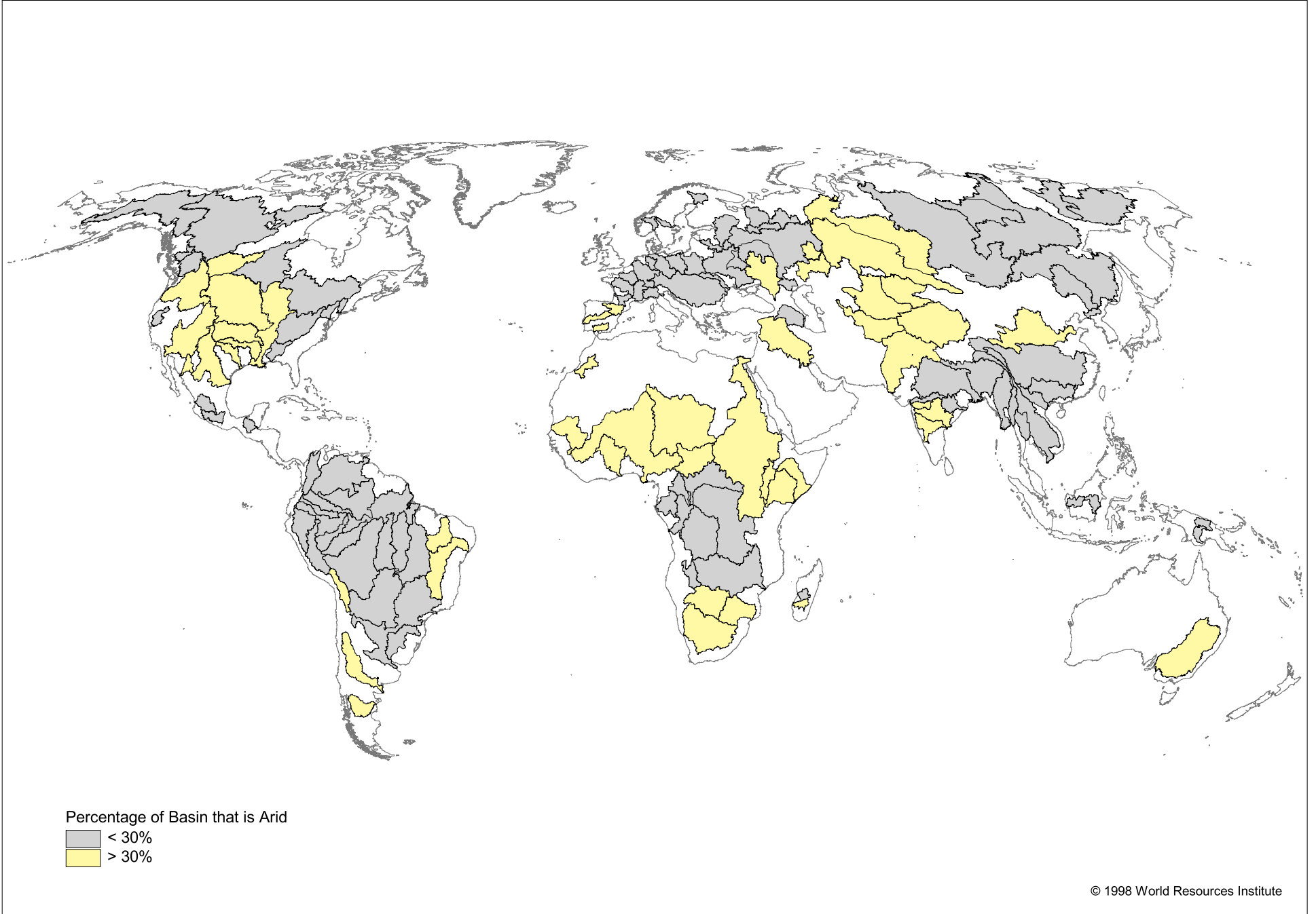
Map 4: Aridity
