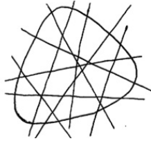
FIGURE 1. A hyperplane tessellation of a set in the plane
