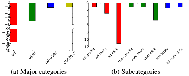
Figure 7: Negated percentage of NRIg diminished when removing features of a particular category.
