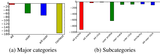
Figure 8: Negated percentage of NRIg diminished when keeping features of a particular category.
