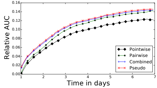
Figure 4: Relative AUC of one week excluding the first day.
