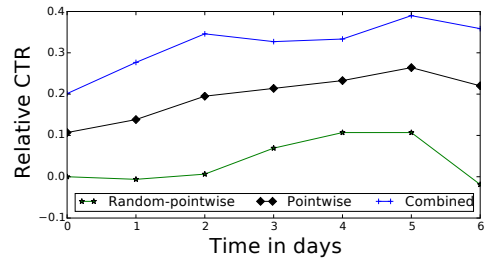
Figure 11: Relative CTR as a function of time.
