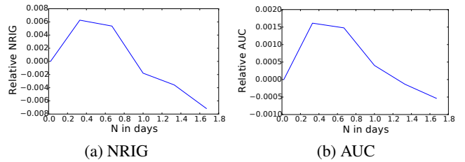
Figure 6: Change of performance against N.
