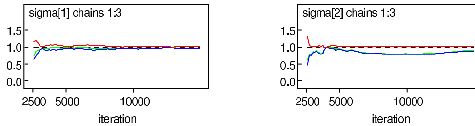
(a) B-G-R Diagnostic Plots for variances
