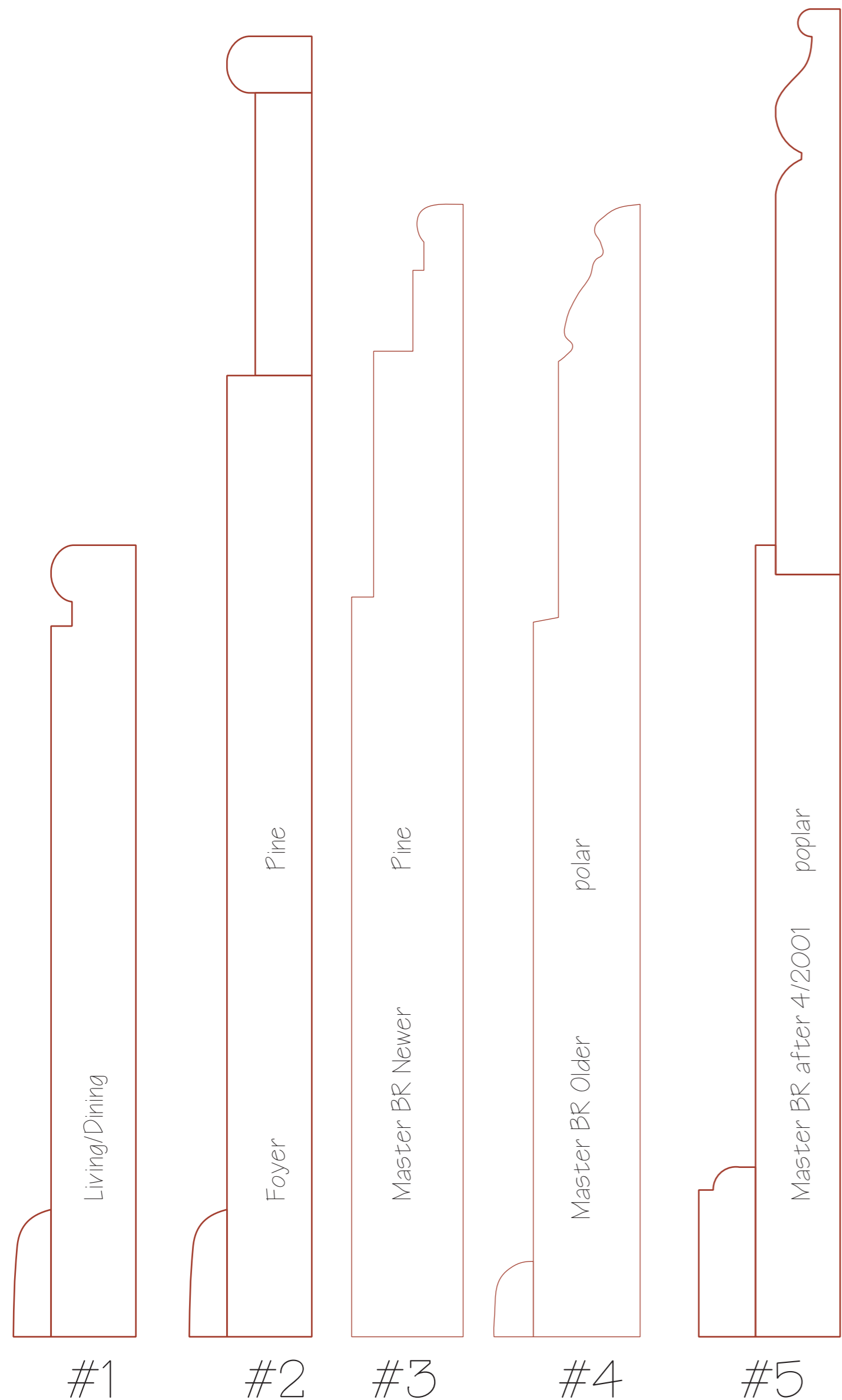
Baseboards
