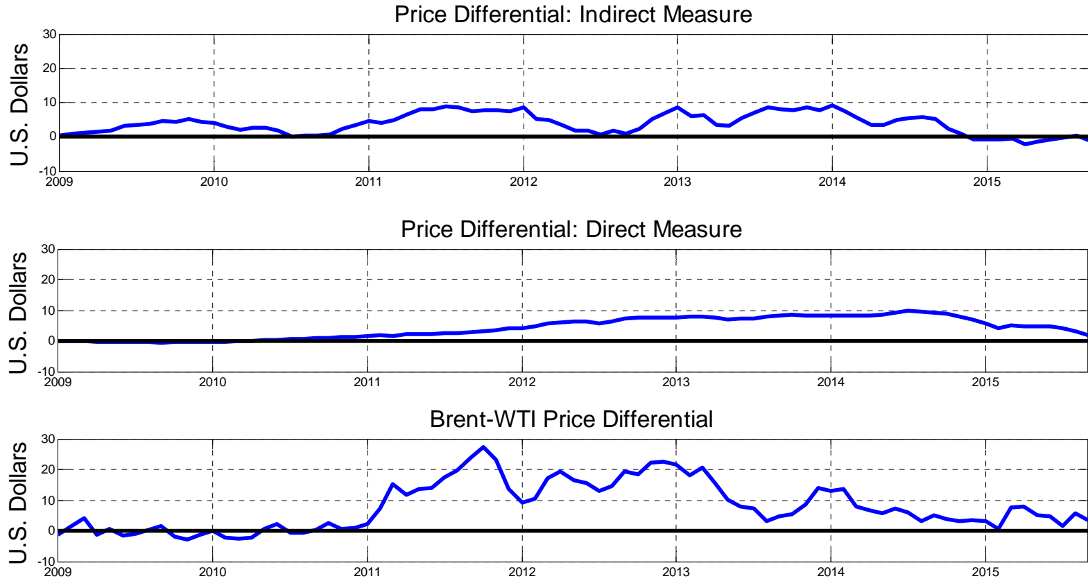
Figure 10. Brent Oil Price Differentials
