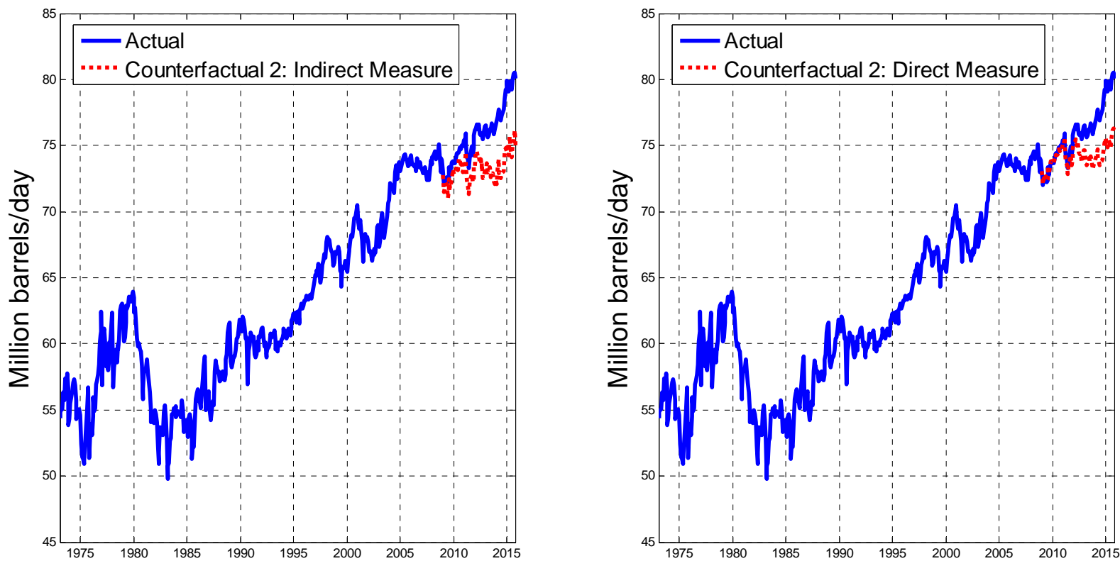
Figure 7. Alternative Counterfactuals for World Oil Production in the Absence of the U.S. Fracking Boom
