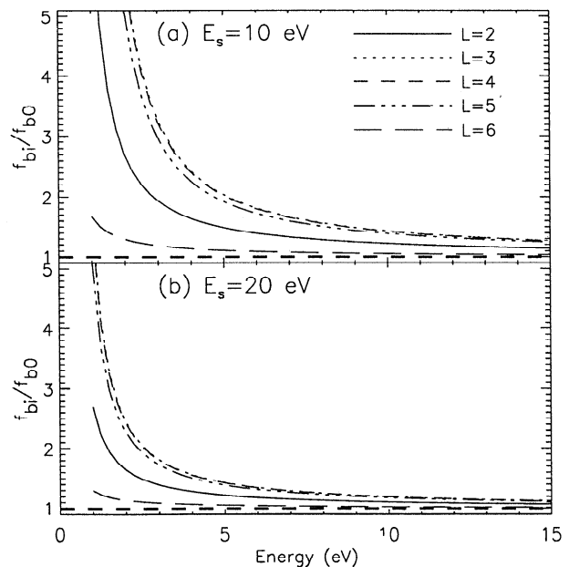
Figure 2. Ratios of topside ionosphere values to magnetic equator values of the electron distribution function at the loss cone-trapped zone boundary at various L shells. Flux ratios are from the solution of (12), with (top) E_s=10 eV (bottom) and 20 eV. The relevant parameters given in Table 2. A heavy dashed line at unity is shown for reference.
