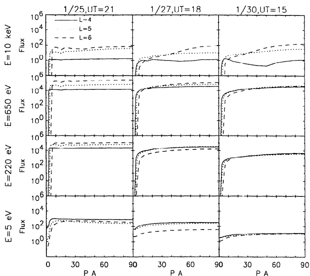
Figure 12. Local midnight plasma sheet electron pitch angle distributions at various energies and simulations times for late January 1991, shown at L =4 (solid line), 5 (dotted line), and 6 (dashed line).
