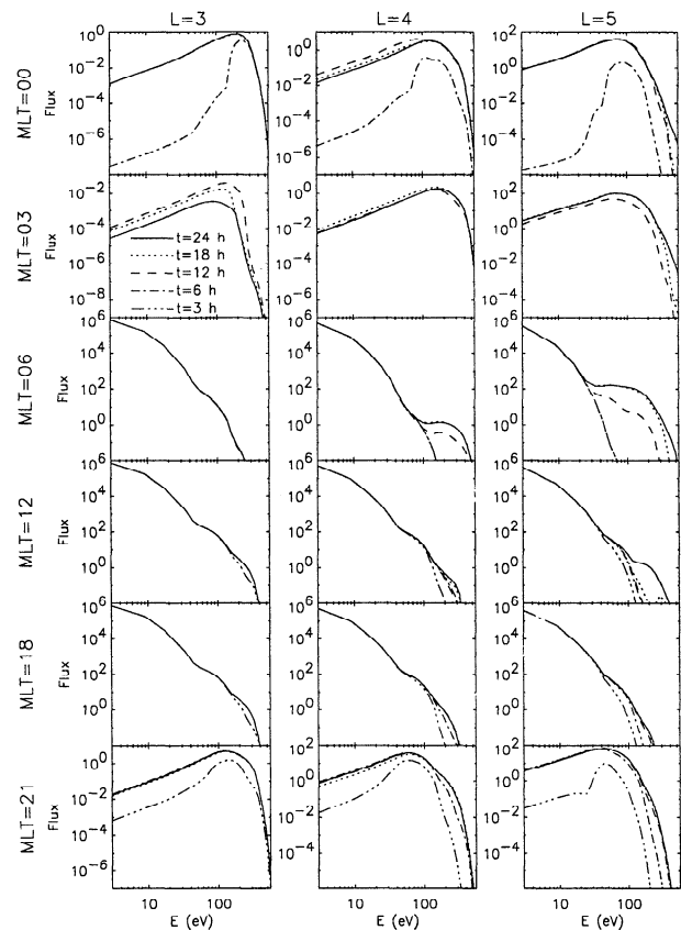
Figure 5. Time development of the 90^\circ equatorial pitch angle energy spectra at various spatial locations in the inner magnetosphere. Simulation times are in hours from photoelectron source turn-on in the dayside ionosphere, with constant Kp=1 geomagnetic activity. Note that each subplot has its own dynamic range. Here and elsewhere, the axis label "flux" refers to differential number flux in (\text{eV cm}^2 \text{s sr}^{-1}) .
