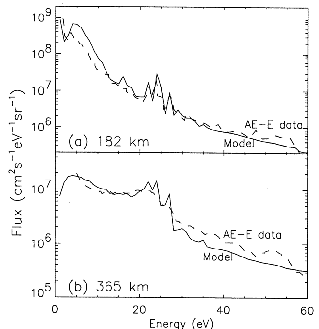
Figure 3. Comparison of model results (solid lines) with AE-E data (dashed lines) at (a) 182 km and (b) 365 km on day 355 of 1975. The satellite data are reproduced from Doering et al. [1976].
