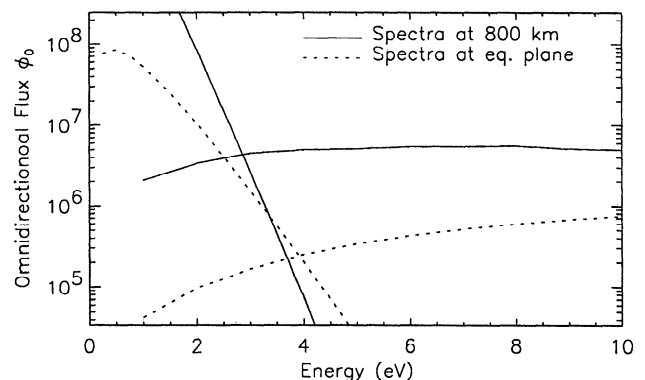
Figure 1. Omnidirectional fluxes for a Maxwellian thermal plasma and modeled photoelectrons at two altitudes along an L=4 flux tube. Thermal plasma parameters are given in Table 1.
