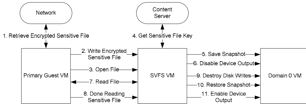
Figure 3. Architecture of the VOFS Client
