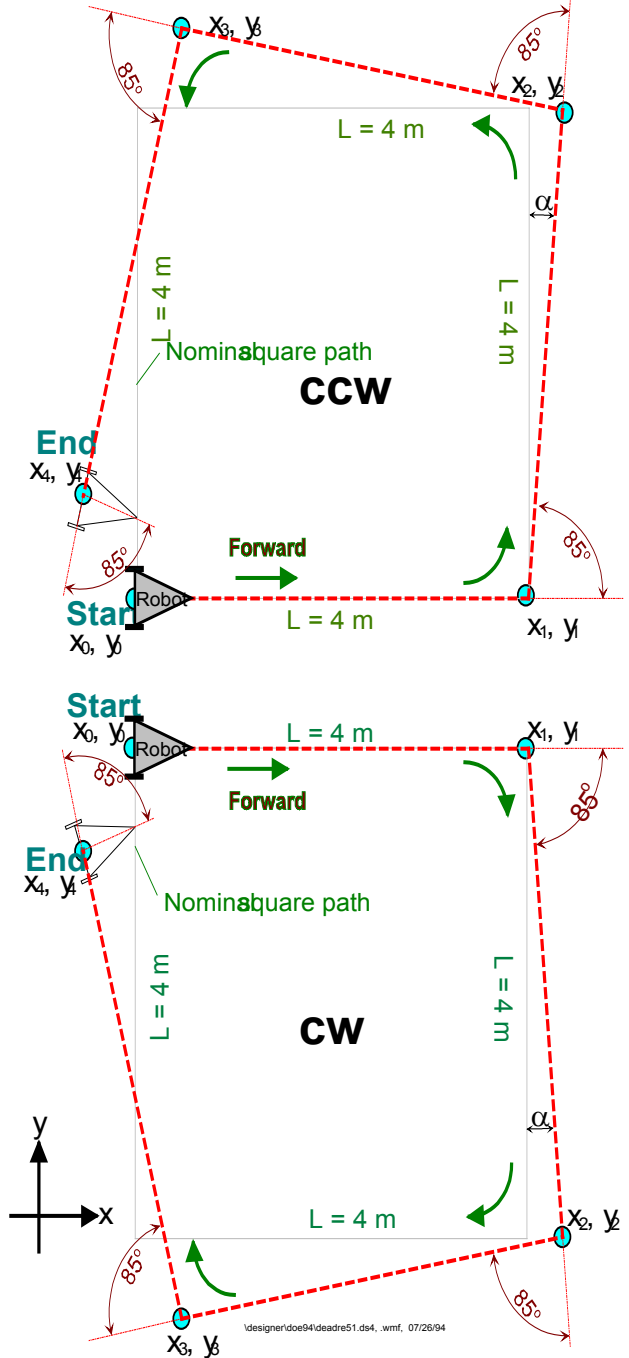
Figure 7: Type A errors in ccw and cw direction. Type A errors are caused only by the wheelbase error E_b .
