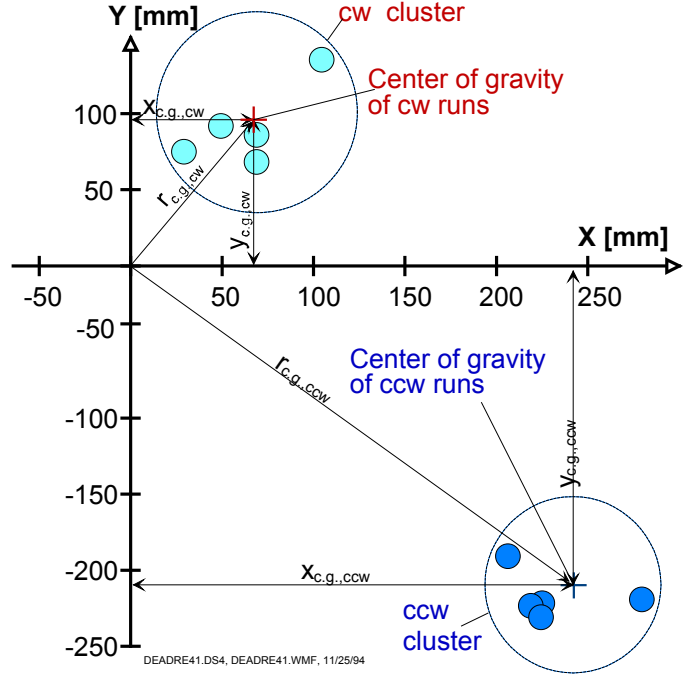
Figure 5: Typical results from running UMBmark (a square path run in both cw and ccw directions) with an uncalibrated vehicle.
