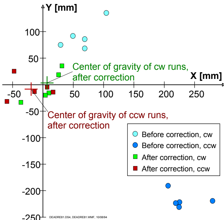
Figure 11: Position Errors after completion of the Bi-directional Square Path Experiment (4 x 4 m). Before calibration: b=340.00 mm, D_R/D_L = 1.00000 After calibration: b=336.17 mm, D_R/D_L = 1.00084
