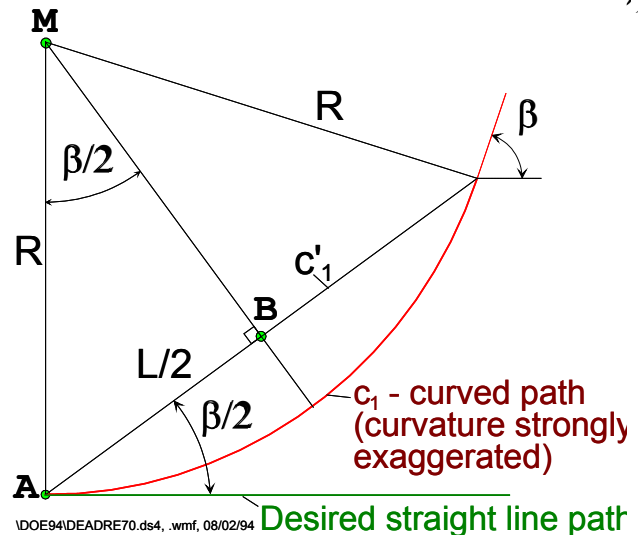
Figure 9: Geometric relations for finding the radius of curvature.
