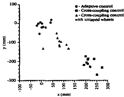
Fig. 9 Motion control accuracy
