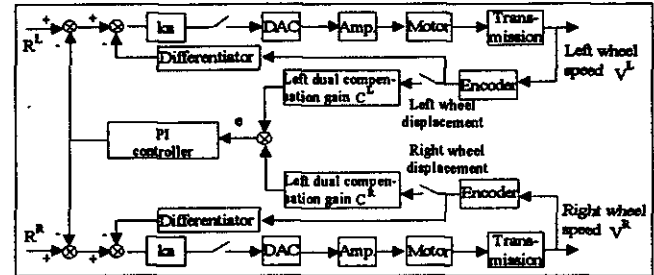
Fig. 3 Cross-coupling motion controller
