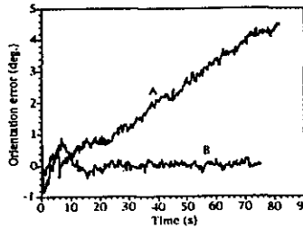
Fig. 8(a) Robot orientation error A - without compensation B - with compensation
