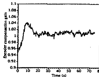
Fig. 8(b) Convergence of the encoder compensation gains
