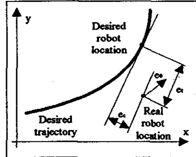
Fig. 1 Motion error decomposition
