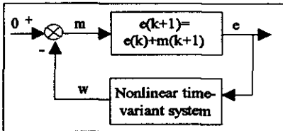
Fig. 6 Resultant equivalent feedback system
