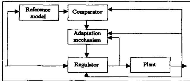
Fig. 2 A model-reference adaptive control system
