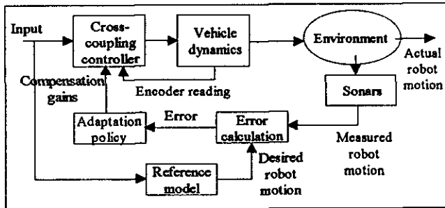
Fig. 4 Proposed adaptive motion control system
