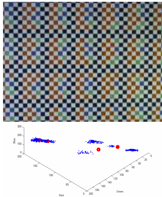
Figure 3: Colour clustering using K-means with random initial conditions. (Top) Example image with five colours. (Bottom) Plot of grid cell RGB components and detected cluster centres.
