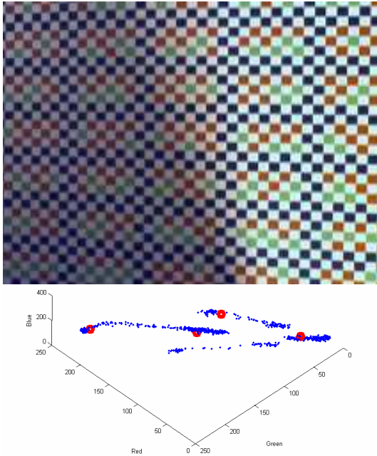
Figure 4: Colour Clustering using K-means with pre-determined initial conditions. (Top) Example image with four colours. (Bottom) Plot of grid cell RGB components and detected cluster centres.
