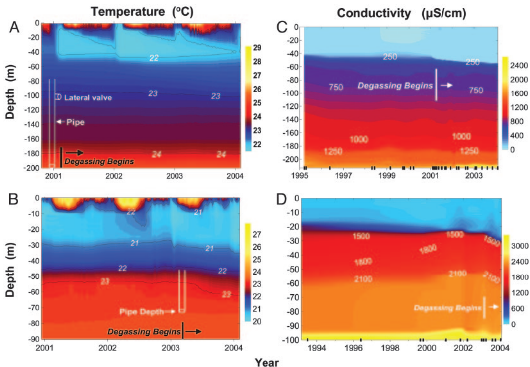
Fig. 2. Time course of changes in temperature (A and B) in Lake Nyos (A) and Lake Monoun (B) and in conductivity (C and D) in Lake Nyos (C) and Lake Monoun (D), showing the depth of degassing pipe openings and the start of degassing. Marks on x axis of C and D indicate sampling dates; sampling in A and B was hourly.
