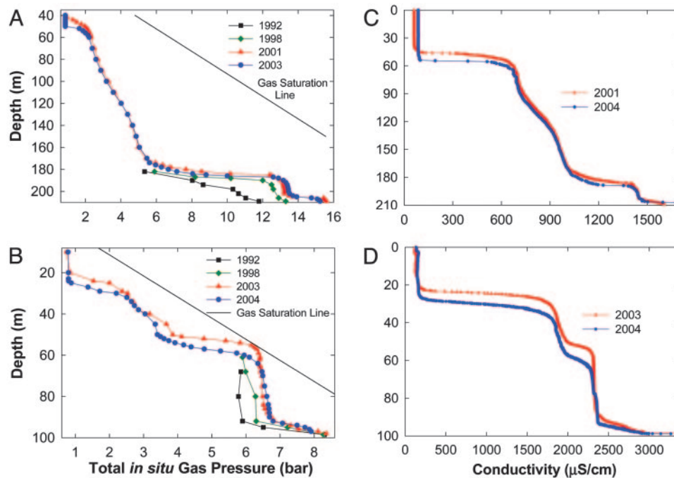
Fig. 1. Depth distribution of total in situ gas pressure (A and B) and conductivity (C and D) in Lakes Nyos (A and C) and Monoun (B and D) over time [1992 = black squares; 1998 = green diamonds; 2001 (Nyos) and 2003 (Monoun) = just before degassing, red triangles; 2004 = postdegassing, blue circles]. The gas saturation line (total hydrostatic plus atmospheric pressure) indicates the bubble-point pressure at which dissolved gas will form bubbles.
