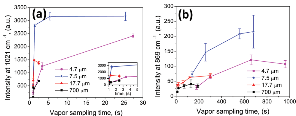
Figure 4. (a) SERS intensity at 1021 cm -1 (symmetric ring breathing mode) of pyridine and (b) SERS intensity at 869 cm -1 (C–H out-of-plane bending mode) of 4-nitrophenol varies with vapor pumping time at room temperature open space using different sizes of capillaries [ID = 4.7 μm (pink circle), 7.5 μm (blue star), 17.7 μm (red triangle), and 700 μm (black square)]. Insert: Enlarged portion of pyridine detection during the first 5 s. Error bars were obtained from three sets of each capillary. The Raman measurements were done at 785 nm, 12 mW laser power, and acquisition time of 2 s.
