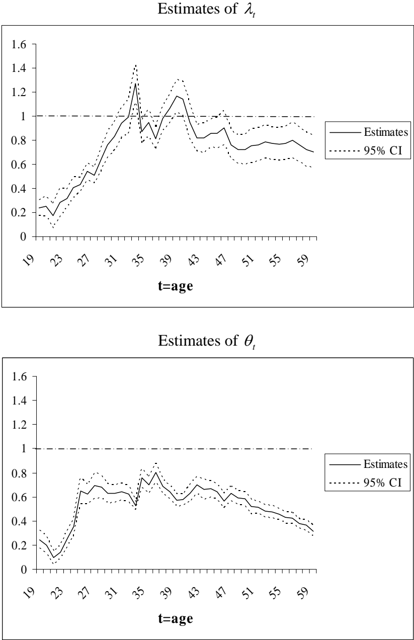
Figure 2. Main Estimates of \lambda_t and \theta_t
