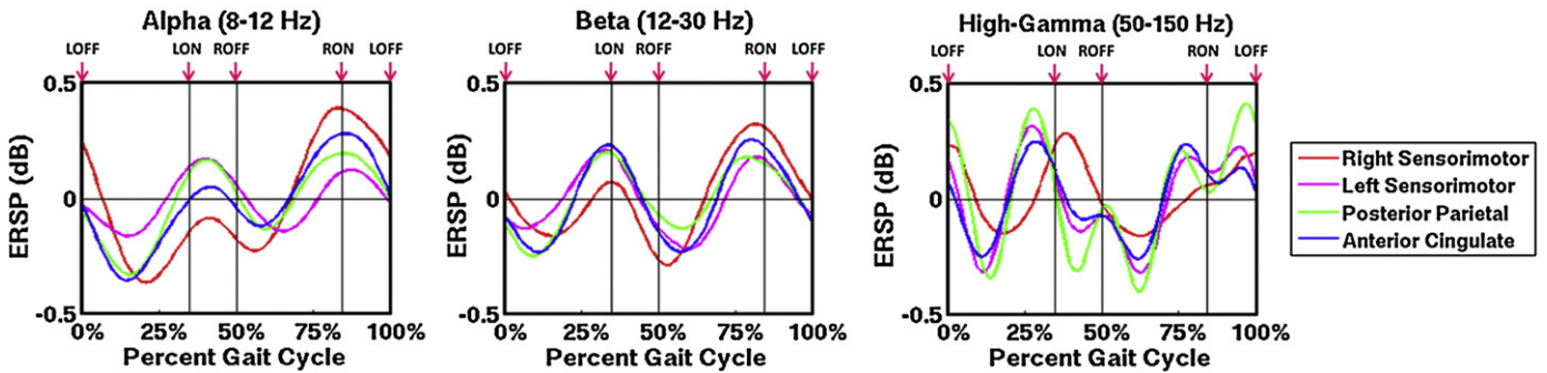
Fig. 3. Average gait event-related spectral perturbation (ERSP) line plots showing the average gait ERSP for the (left) alpha (8–12 Hz), (middle) beta (12–30 Hz), and (right) high-gamma frequency bands. Each cluster of electrocortical sources is represented by a colored trace: (red) right sensorimotor cluster, (magenta) left sensorimotor cluster, (green) posterior parietal cluster, and (blue) anterior cingulate cluster. The gait cycle begins and ends with left toe-off (LOFF). Vertical lines indicate the timing of left heel-strike (LON), right toe-off (ROFF), and right heel-strike (RON).
