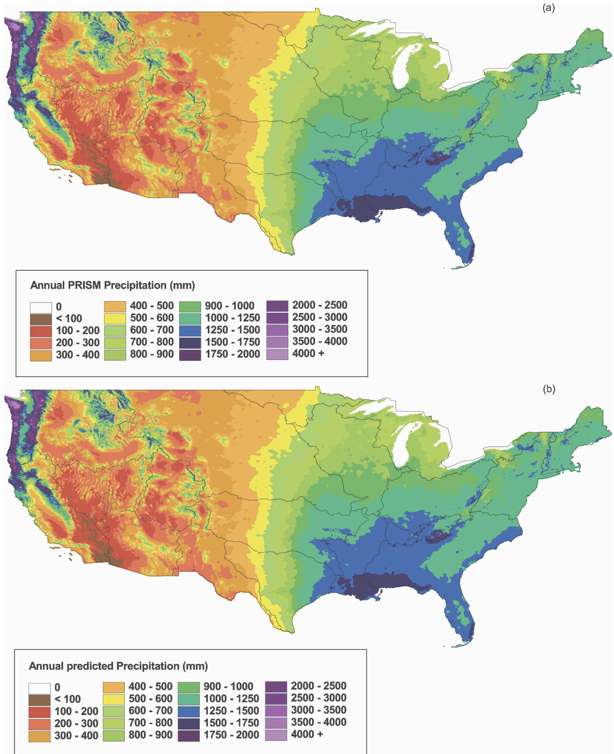
FIG. 7. Annual average (a) PRISM and (b) predicted precipitation accumulated in the period 1960–2001. (c) Cell-by-cell difference between predicted and PRISM average annual precipitation (PRISM subtracted from the predicted) as a percentage of PRISM in the period 1960–2001.
