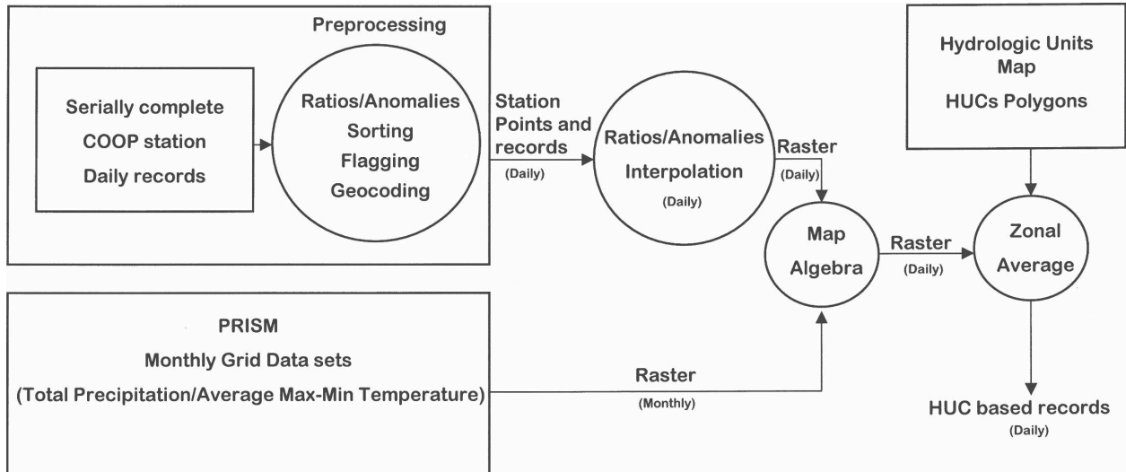
FIG. 5. Scheme of the input–output data elaboration.
