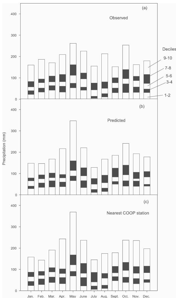
FIG. 13. Monthly accumulated precipitation deciles (a) observed at the TX-RG69 station, (b) predicted, and (c) observed at the nearest COOP station.
