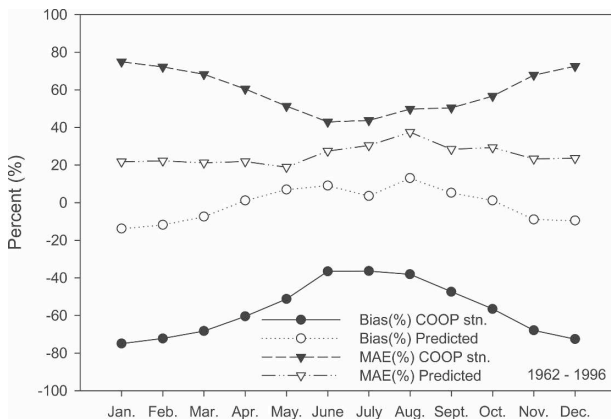
FIG. 10. As in Fig. 9, but for the ID-163x20 station.
