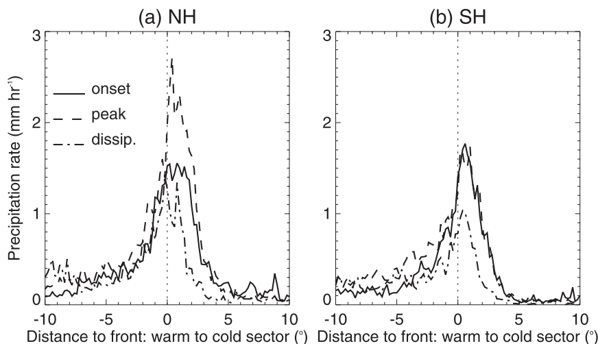
FIG. 11. CloudSat precipitation rate across warm fronts, for cyclone onset (solid), peak (dashed) and dissipation (dotted–dashed) in (a) NH and (b) SH. The dotted line marks the position of the surface front.
