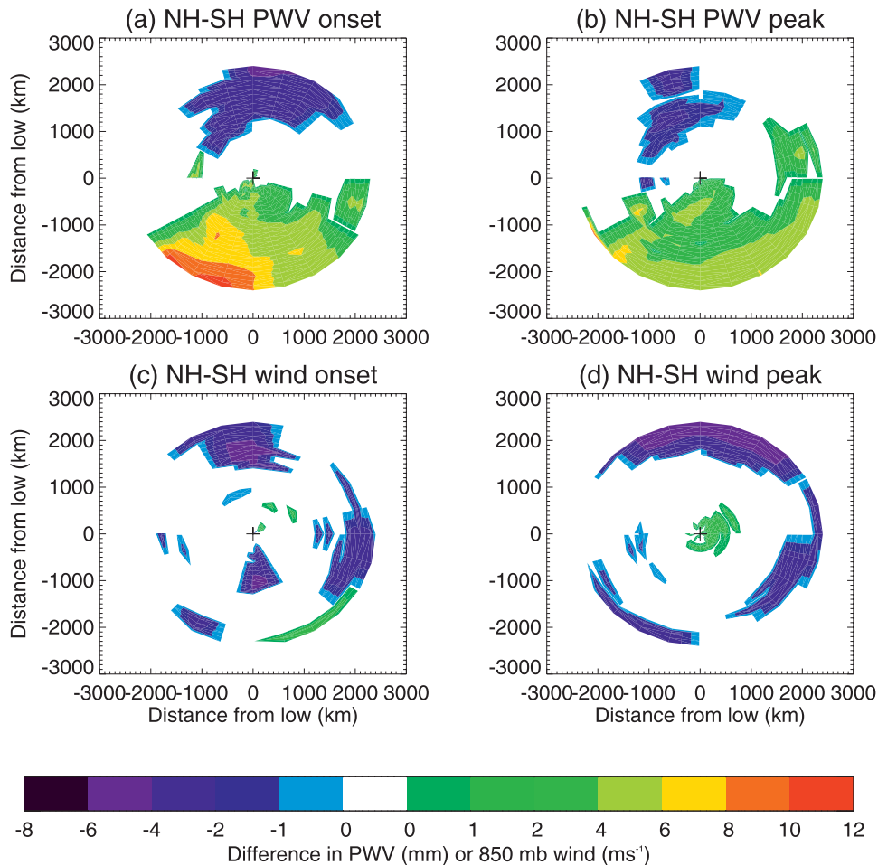
FIG. 5. Difference NH – SH in (a),(b) AMSR-E PWV and (c),(d) MERRA 850-mb wind speed at cyclone (a),(c) onset and (b),(d) peak when significant at the 95% level.
