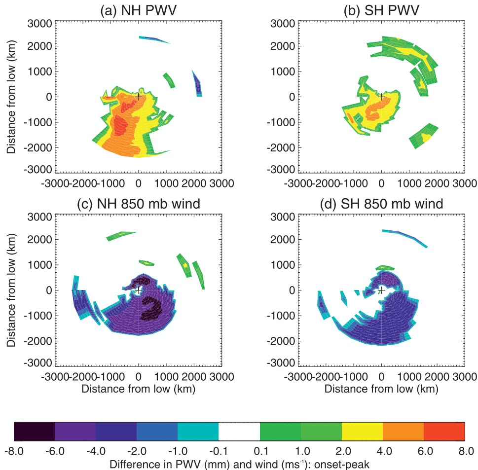
FIG. 6. Difference in (top) AMSR-E PWV and (bottom) MERRA 850-mb wind speed between cyclone onset and peak in (a),(c) NH and (b),(d) SH when significant at the 95% level.
