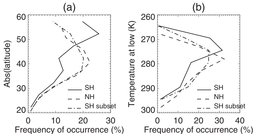
FIG. 1. Distribution of (a) cyclone centers as a function of absolute latitude in the NH (dashed) and SH (solid) midlatitude regions and (b) temperatures at the low pressure center. The dotted–dashed line shows the SH subset distribution obtained by randomly selecting SH cyclones in 5^\circ latitude bands until their number matches the NH dataset.
