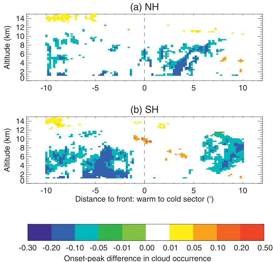
FIG. 12. Difference in CloudSat – CALIPSO cloud occurrence when significant at the 95% level between cyclone onset and peak in (a) NH and (b) SH. The dashed line marks the position of the surface front.
