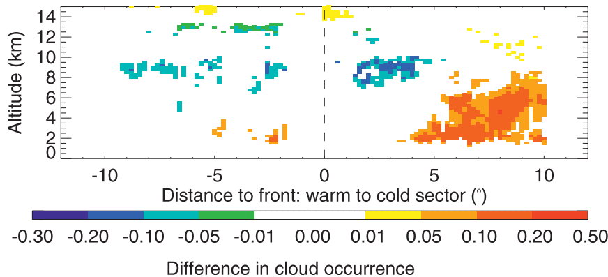
FIG. 10. Difference in CloudSat – CALIPSO cloud occurrence when significant at the 95% level at cyclone onset between NH and SH.
