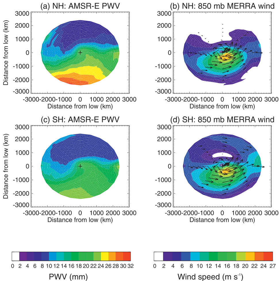
FIG. 13. Composites of (left) AMSR-E PWV and (right) MERRA 850-mb wind for (a),(b) NH and (c),(d) SH. The arrows in (b) and (d) indicate the wind direction, with the size of the arrows proportional to the wind speed.
