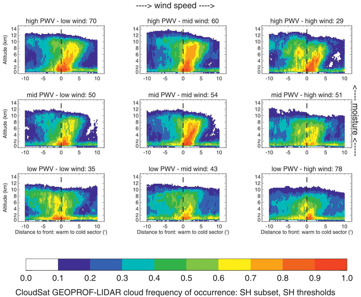
FIG. 9. CloudSat – CALIPSO cloud frequency of occurrence across warm fronts for SH as a function of (left to right) wind speed and (bottom to top) PWV. The number of cyclones per subset is given at the top of each plot.
