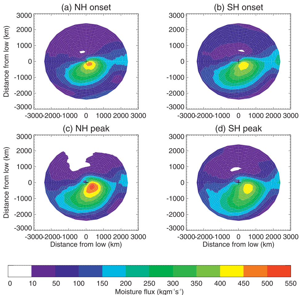
FIG. 4. Moisture flux composites for cyclones at (a),(b) onset and (c),(d) peak in (a),(c) NH and (b),(d) SH.
