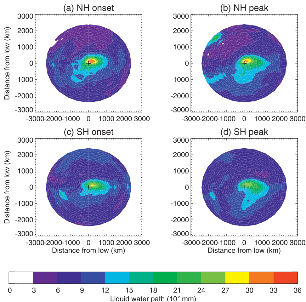
FIG. 8. As in Fig. 7, but for AMSR-E LWP composites.
