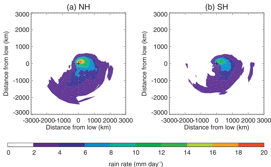
FIG. 16. Composites of AMSR-E precipitation rates for (a) NH and (b) SH.
