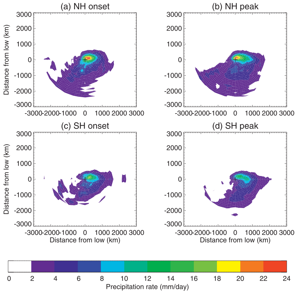
FIG. 7. AMSR-E precipitation rate composites at cyclone (a),(c) onset and (b),(d) peak for (a),(b) NH and (c),(d) SH.
