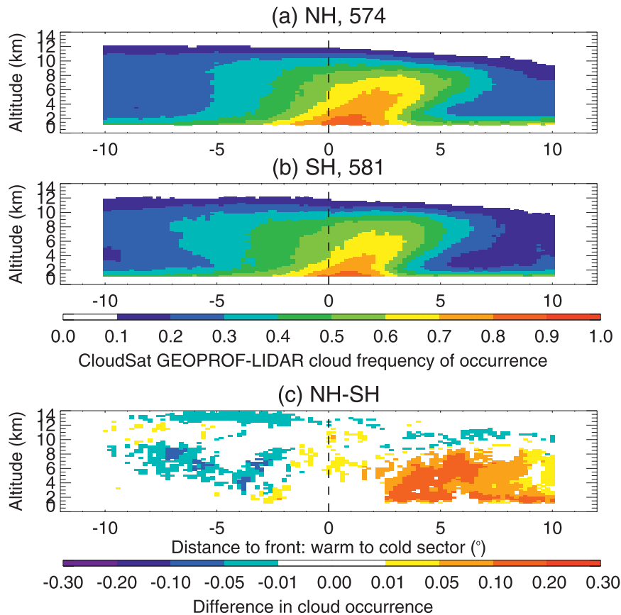
FIG. 14. CloudSat – CALIPSO cloud frequency of occurrence across warm fronts in (a) NH and (b) SH, with (c) difference in cloud occurrence between NH and SH when significant at the 95% level based on a binomial statistical test. The x axis represents the distance in degrees from the surface front indicated by the dashed line. Positive values are in advance of the front and negative values in the warm sector.
