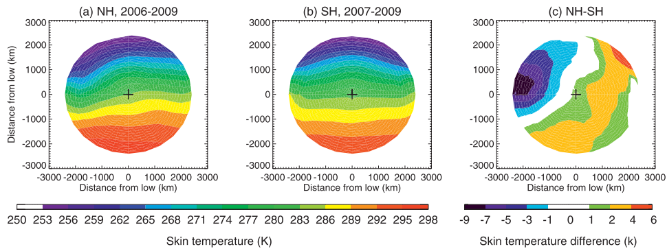
FIG. 3. Composite of MERRA skin temperature centered on cyclone low pressure for (a) NH and (b) SH subset cyclones; (c) difference in skin temperature composites between NH and SH cyclones.
