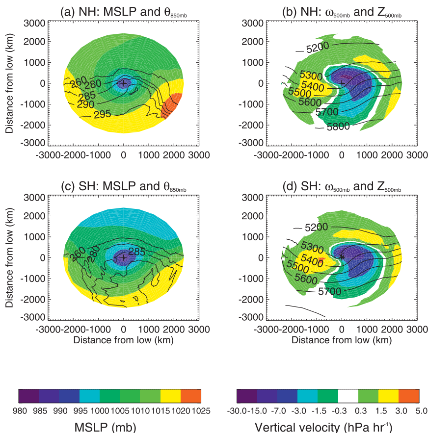
FIG. 2. Composites of (left) MERRA SLP with \theta_{850\text{mb}} and (right) \omega_{500\text{mb}} with Z_{500\text{mb}} for (a),(b) NH and (c),(d) SH cyclones. Each field is rotated to align the warm front along the x axis, and the rotation angles are similarly distributed between the two hemispheres. The north-south axis is flipped for SH cyclones.
