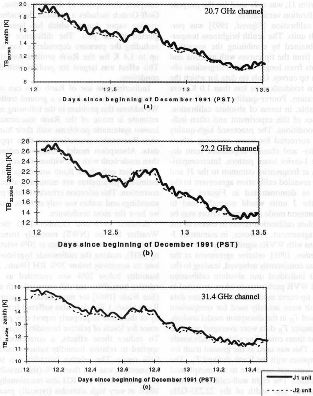
Figure 3. Zenith brightness temperature intercomparison for radiometer units J1 and J2 during December 1991 at San Diego, California, at (a) 20.7 GHz, (b) 22.2 GHz, and (c) 31.4 GHz. Measurements have been smoothed by a 30-min running average.
