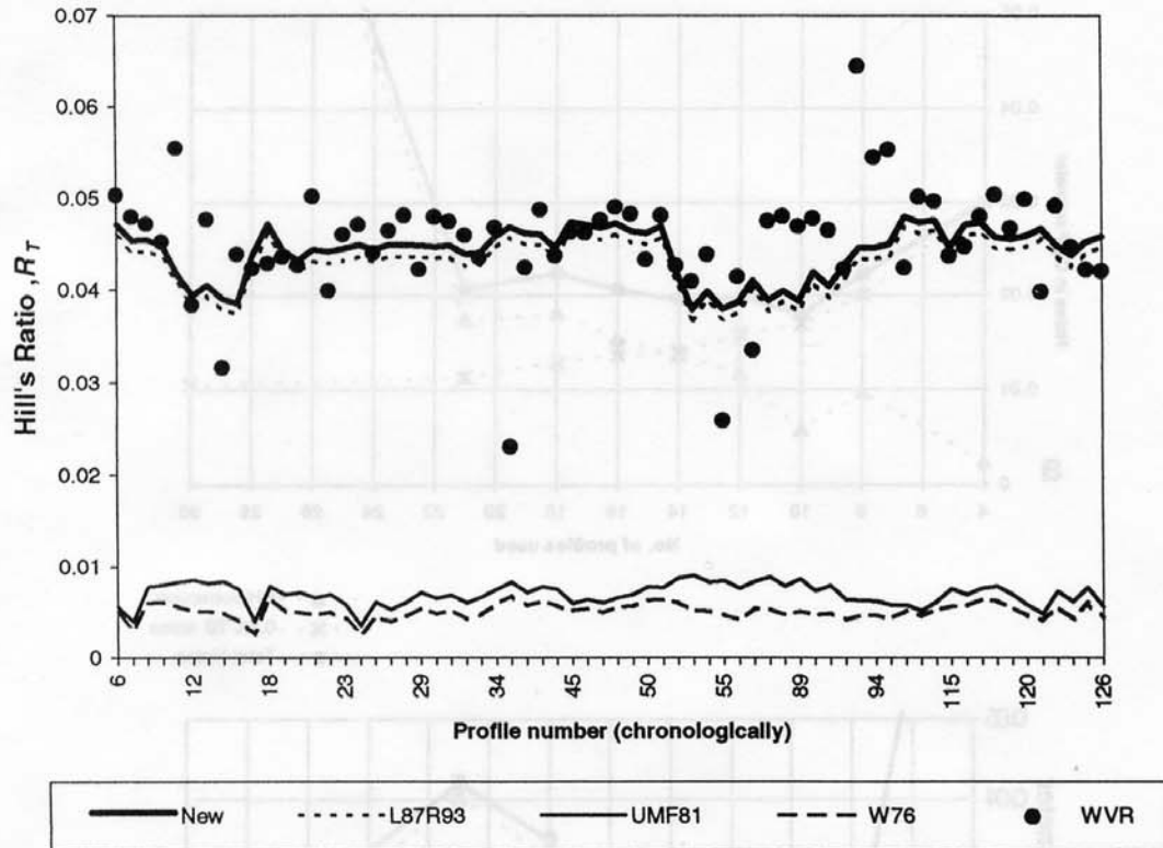
Figure 5. Hill ratio comparison between various atmospheric models, showing agreement of the chosen water vapor line shape with the radiometer data (see text for explanation of model acronyms).
