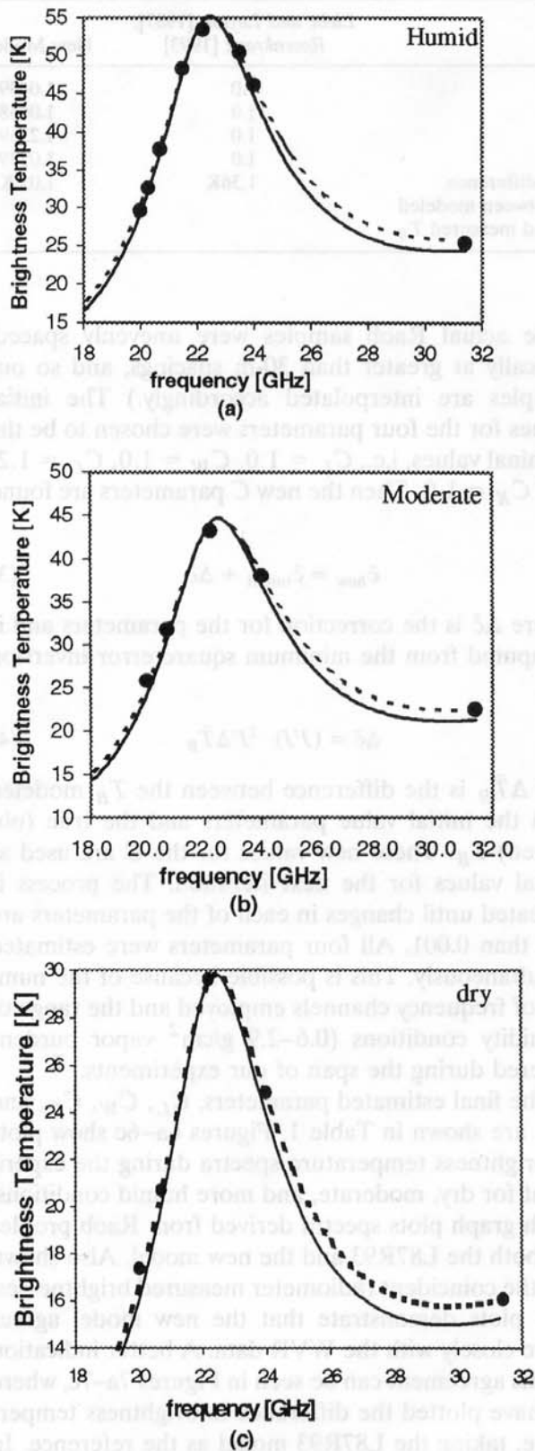
Figure 6. (opposite) Brightness temperature spectra comparison between water vapor radiometer (WVR) data and radiosonde-derived data with new and nominal parameters for a vapor burden of (a) 2.9 g/cm 2 , (b) 2.3 g/cm 2 , and (c) 1.3 g/cm 2 . (Note that only five channels were in operation during the Raob launches for the conditions in Figures 6b and 6c. Solid lines show the L87R93 model, dotted lines show the new model, and the solid dots show the WVR data.
