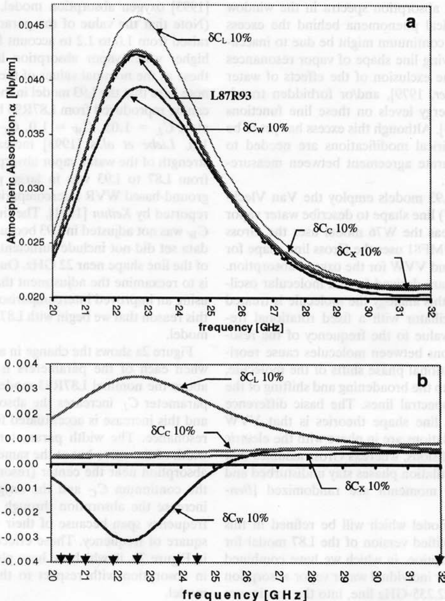
Figure 2. (a) Effect of line parameter variation by 10% on total atmospheric absorption. (b) Differential effect of line parameter variation with respect to nominal L87R93 (L87 combined with Rosenkranz [1993]) model. The arrows at the bottom of the figure indicate the frequencies measured in this experiment. (Atmospheric conditions are the same as in Figure 1.)
