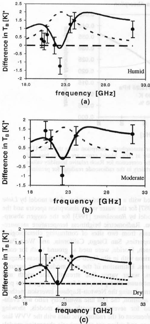
Figure 7. Plot of the difference T_B - T_{BL87R93} for (a) humid (West Palm Beach), (b) moderate (San Diego), and (c) dry (San Diego) conditions. Note that the Liebe and Layton [1987] T_B is equivalent to our nominal model ( C_L = C_W = C_X = 1.0 and C_C = 1.2 ). (Only five channels were in operation during the Raob launches for the conditions in Figures 7b and 7c.) Dashed lines show the L87R93 model, dotted lines show the L93 model, solid lines show the new model, and solid dots show the WVR data.
