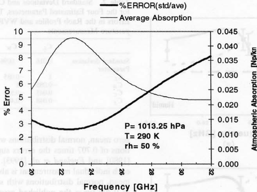
Figure 8. Percentage error in the improved model for atmospheric absorption using the 1962 U.S. Standard Atmosphere at sea level with relative humidity at 50%. Model errors are due to bias and random measurement uncertainties in radiometer T_B , the correction for Raob relative humidity values less than 20% or greater than 100%, and the bias uncertainty in the radiosonde readings for pressure, temperature, and relative humidity.
