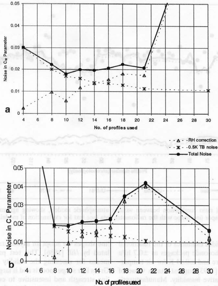
Figure 4. Total error in (a) C_W and (b) C_L line parameters due to a 0.5-K uncertainty in measured T_B and the correction of the Raob relative humidity reading versus number of Raob profiles used in the estimation (see section 3.2 for a complete discussion). A trade-off between the amount of data used and the minimum error in parameter estimation yields an optimum value of 21 Raob profiles, providing a total of 108 data points at individual frequency channels.
