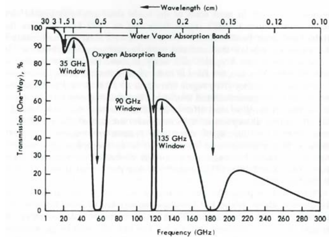
Fig. 1.6: Percentage transmission through the earth's atmosphere, along the vertical direction, under clear sky conditions. (courtesy [7])
