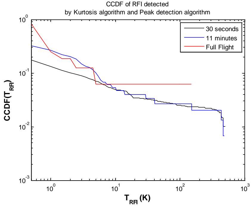
Fig. I.1: CCDF of brightness temperature contribution of all types of RFI detected using the kurtosis and peak detection algorithms
