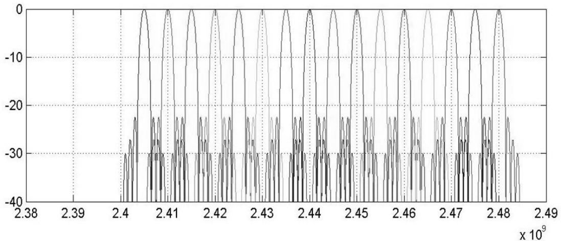
Fig. II.2: Frequency scheme of IEEE 802.15.4 communication standard [86]
