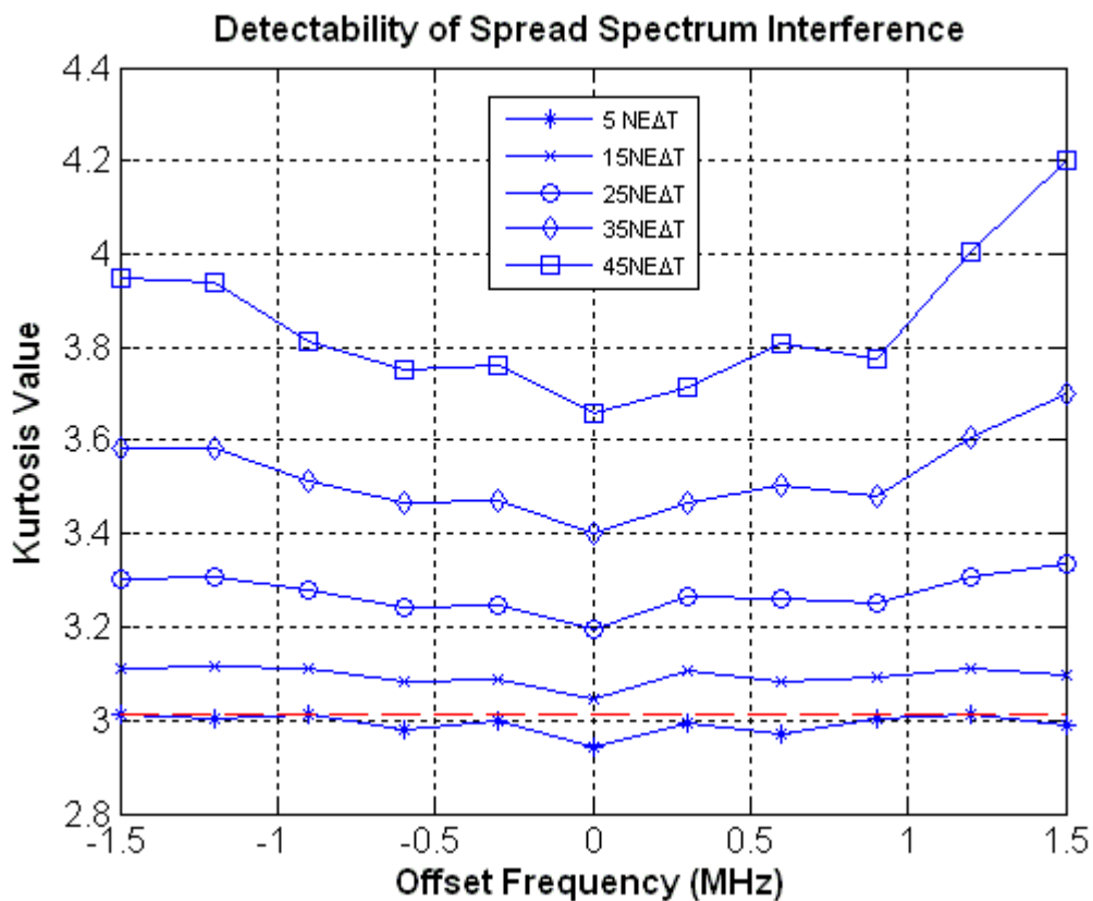
Fig. II.5: Kurtosis values when the spread spectrum signal is offset in frequency from the center of sub-band 4 of ADD. The straight line represents the kurtosis detection threshold
