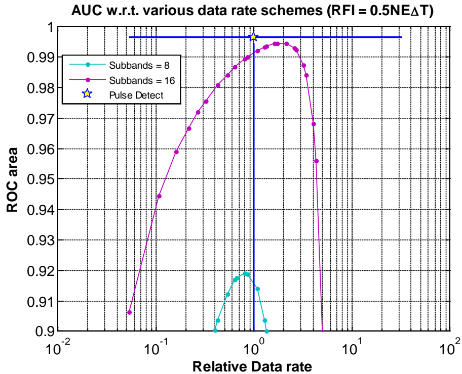
Fig. 3.3: (a) Plot comparing the ROC area for the kurtosis algorithm as a function of relative data rate and number of sub-bands with the matched pulse detection algorithm (star) (b) Magnified plot indicating ROC area of the kurtosis algorithm near matched pulsed detection algorithm (star) (RFI power = 0.5NE \Delta T). The relative data rate is with respect to the ideally matched pulse detector. Heavy blue lines represent data rate and ROC area values for the matched pulse detector.
