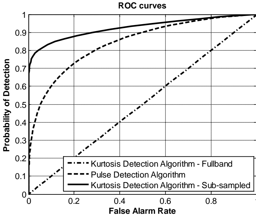
Fig. 3.2: Plot of the ROC curves for three RFI detection schemes (Pulse-detection algorithm, Fullband kurtosis detection algorithm, Sub-sampled kurtosis algorithm) for a 0.33% duty-cycle pulsed-sinusoid RFI with a 0.5 NEAT power level.
