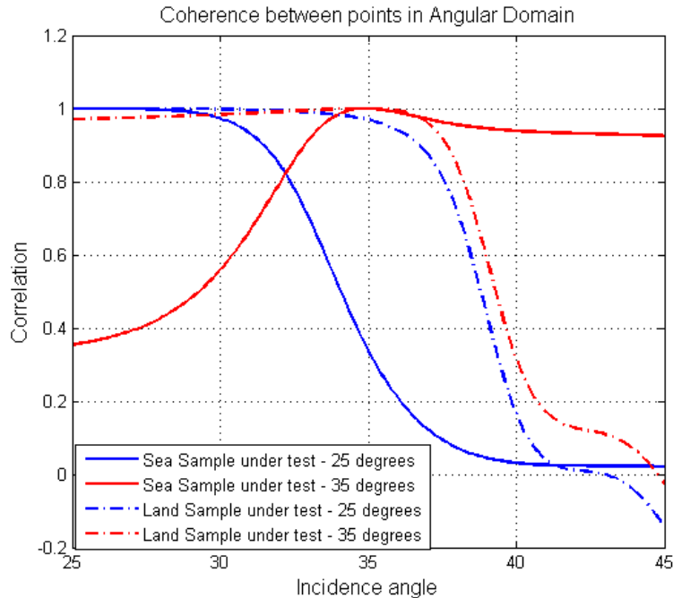
Fig. 5.4: Correlation statistics between an angular domain sample and its neighboring pixels based on two SMOS half-orbits. The blue-curve represents correlation between a sample under test at 25° incidence angle and the red-curve represents a sample under test at 35° incidence angle. The dashed line represents land statistics and solid line represents sea statistics.
