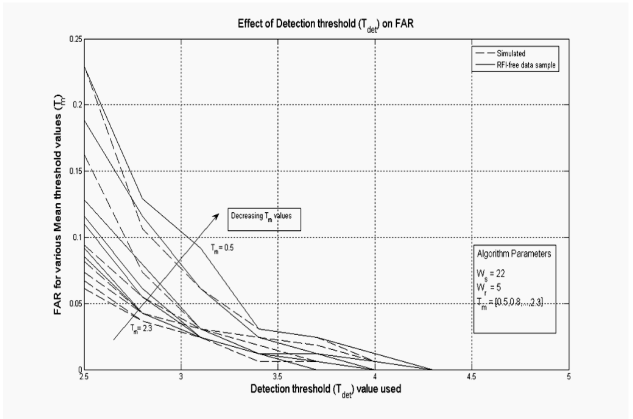
Fig. 2.3: Effect of detection-threshold magnitude, T_{det} on the FAR of the second moment detection algorithm for the mean-threshold magnitude, T_m values (from upper right to lower left): T_m = 0.5, 0.8, 1.1, 1.4, 1.7, 2.0, 2.3 .
