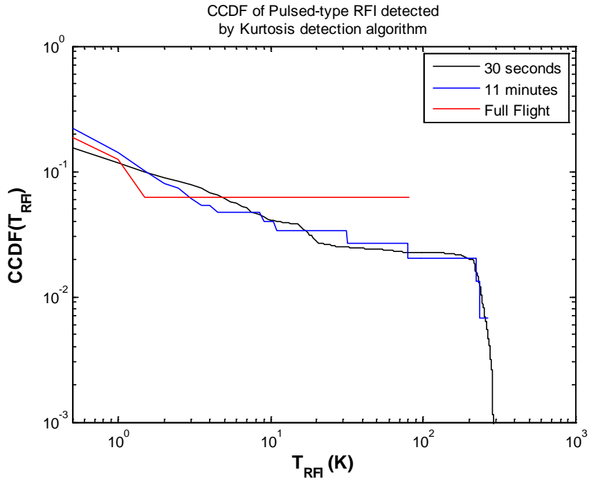
Fig. I.3: CCDF of brightness temperature contribution of pulsed type RFI detected using the kurtosis detection algorithm
