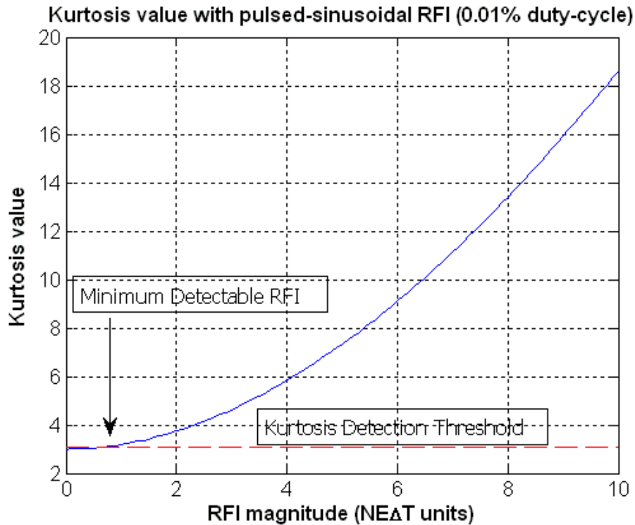
Fig. II.1: Plot indicating change in kurtosis as a function of the RFI magnitude for pulsed-sinusoid interference with a 0.01% duty cycle. The dashed line indicates the kurtosis 3\sigma detection threshold
