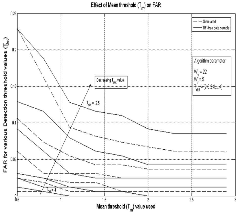
Fig. 2.2: Effect of mean-threshold magnitude, T_m on the FAR of the second moment detection algorithm for the detection-threshold magnitude, T_{det} values (from upper right to lower left): T_{det} = 2.5, 2.8, 3.1, 3.4, 3.7, 4.0 .
