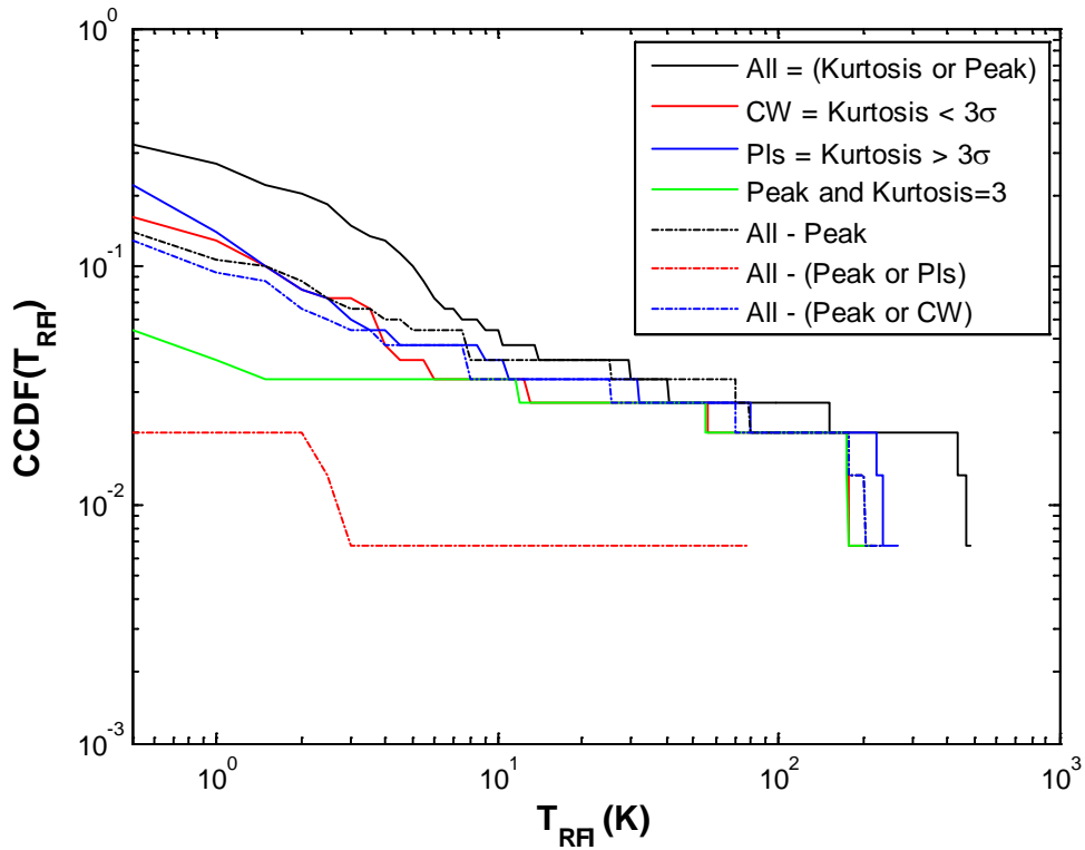
Fig. I.6: CCDF of detected and residual types of RFI brightness temperature contribution for a 11 min integration period
