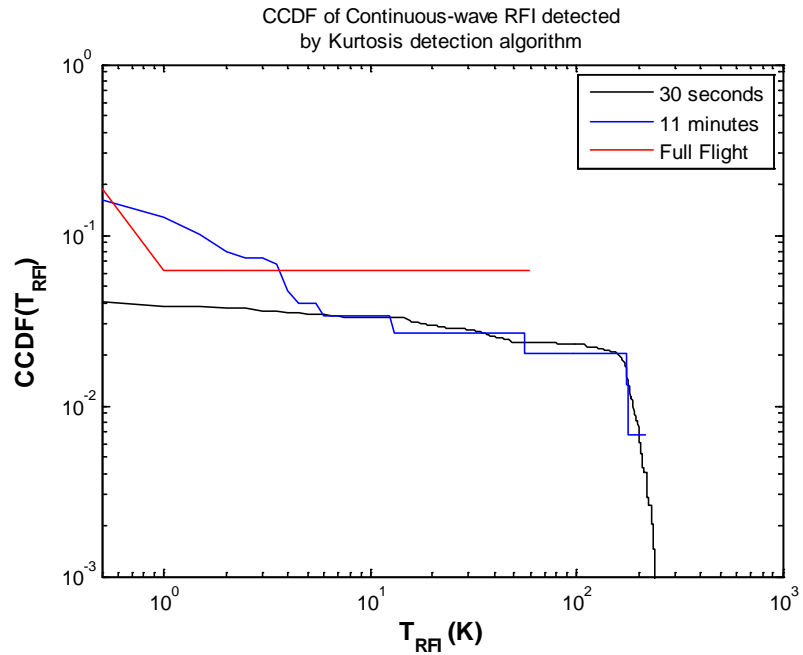
Fig. I.2: CCDF of brightness temperature contribution of continuous wave RFI detected using the kurtosis detection algorithm
