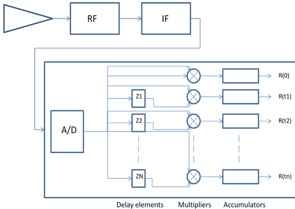
Fig. 6.1: Simplified Block diagram indicating implementation of a digital lag correlator
