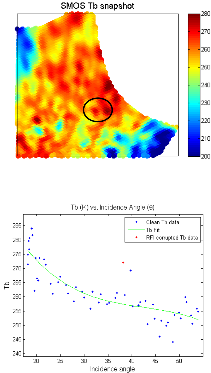
Fig. 5.7: (a) SMOS H-pol Tb snapshot with an indistinct RFI spot within the circle (b) Angular domain representation of the same RFI pixel with flagged RFI Tb (red), RFI-free Tbs (blue) and cubic fit (green).
