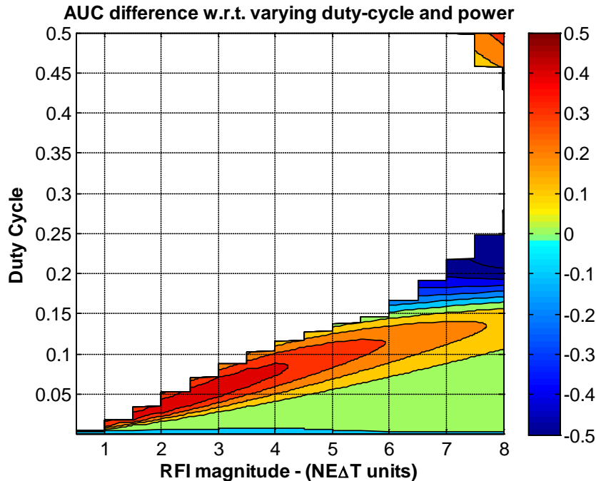
Fig. 3.6: Same as Fig. 3.5 except that the kurtosis detection algorithm has 16 sub-bands and 2 sub-sampling period
