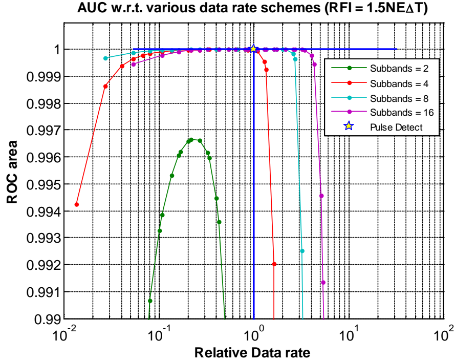
Fig. 3.4: Same as Fig. 3.3 except (RFI power = 1.5NE\Delta T )
