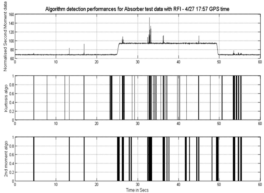
Fig. 2.7: PALS-ADD L-Band radiometer measurements of nadir sky view with BB absorber placed in front of the antenna for a while. (top) 2 nd moment time series; (center) kurtosis of signal; (bottom) Aquarius RFI detection algorithm
