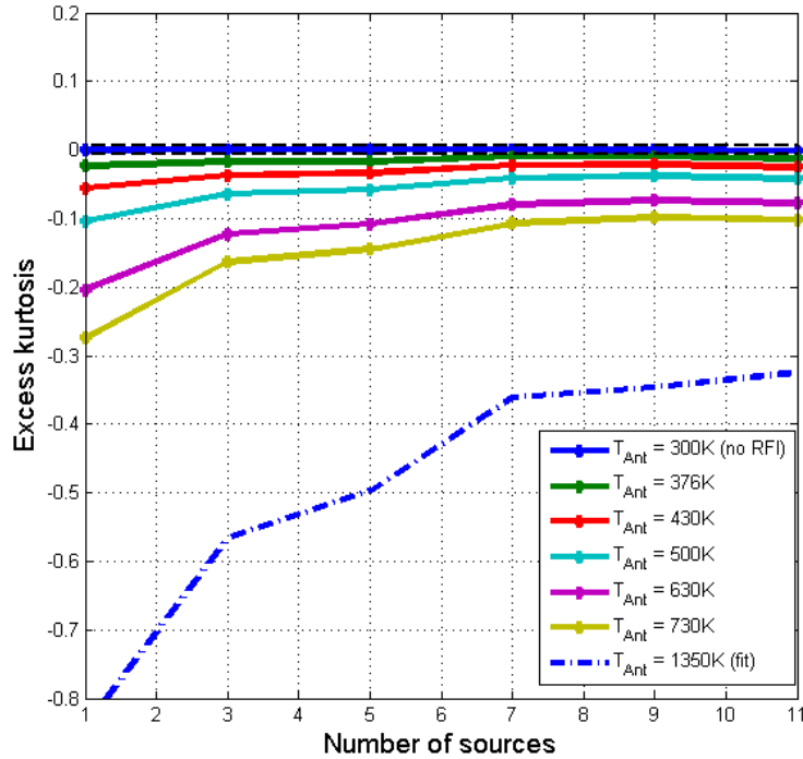
Fig. 4.9: Curves indicating kurtosis variation versus the number of RFI sources for different power levels. The solid lines represent mean kurtosis calculated from experimental data, the dashed curve is fit from the experimental data at 1350K antenna Tb with a 300K background.
