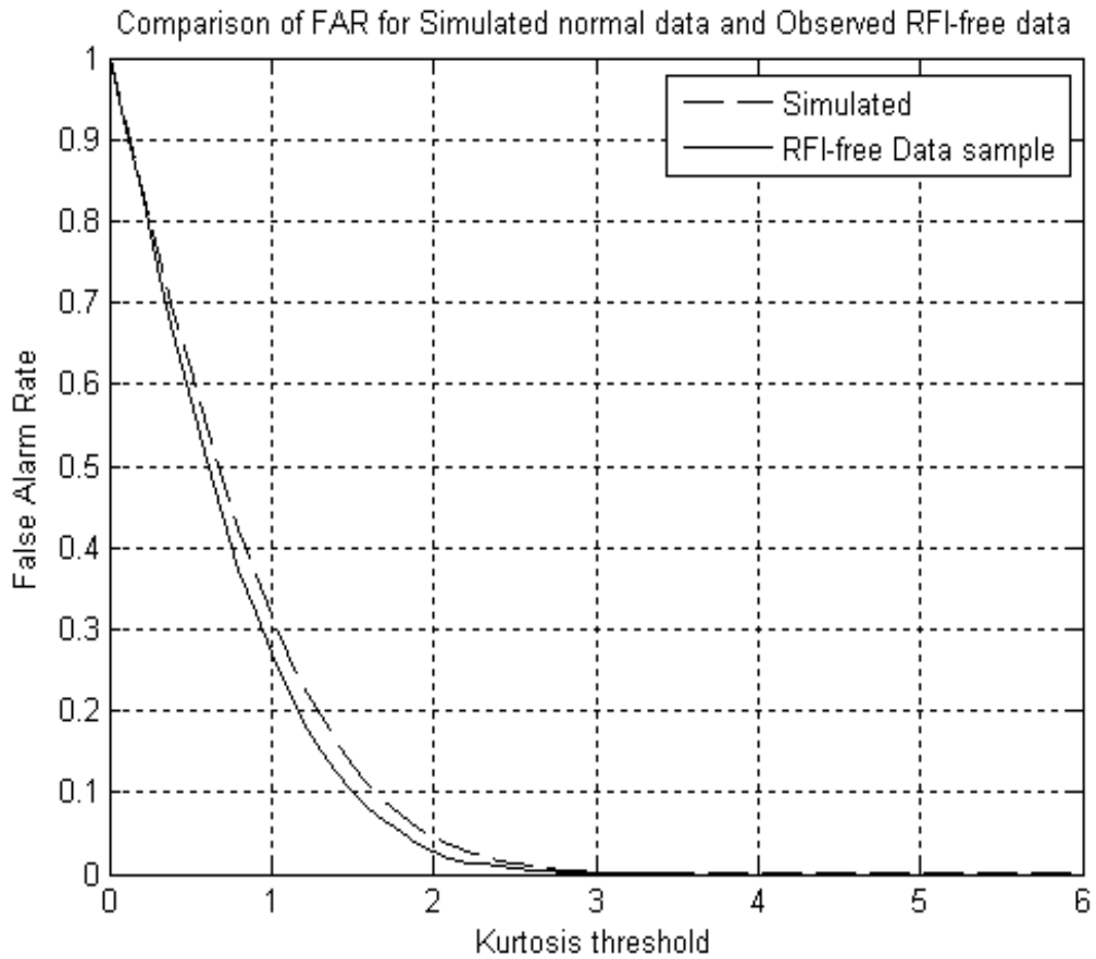
Fig. 2.1: FAR of the kurtosis detection algorithm for various thresholds calculated from normally distributed simulated data (dashed line) and RFI-free PALS-ADD data sample (solid line)
