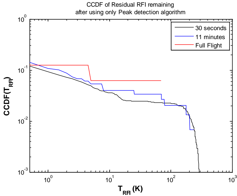
Fig. I.5: CCDF of residual RFI detected using only the peak detection algorithm
