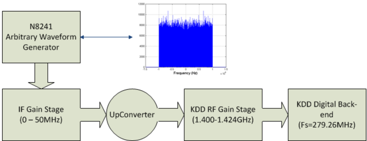
Fig. 4.7: Block-diagram of Multi-source RFI experimental setup
