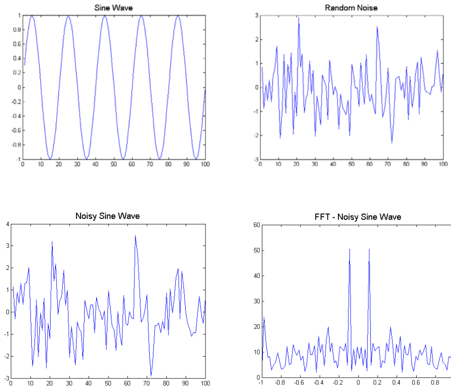
Fig. 5.2: Illustration of (a) Sinusoidal wave in time domain (b) Gaussian noise in time domain (c) combined signals in time domain, representing an indistinguishable noisy sinusoidal wave, and (d) combined signals in frequency domain, with clear peaks distinguishable from the noise floor.
