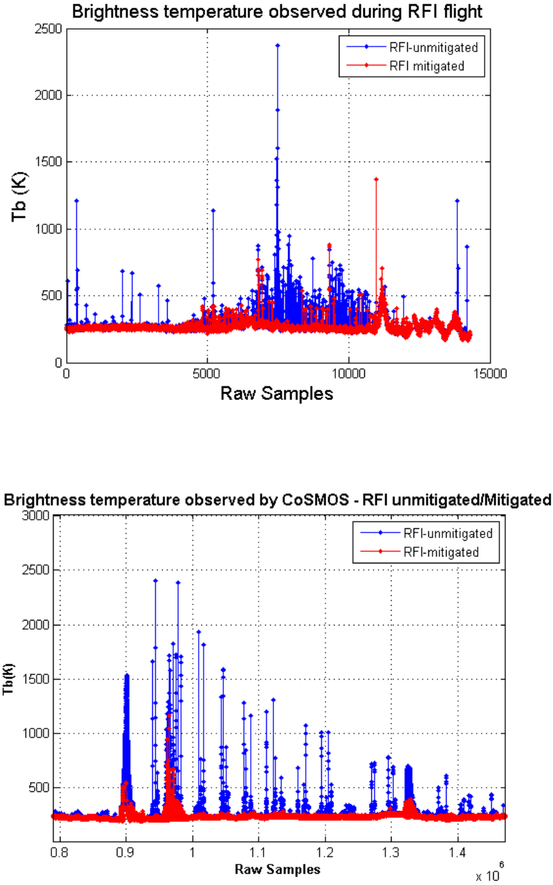
Fig. 4.1: Brightness temperature values over (a) New York – 10ms samples and (b) Central Europe – 8ms samples ( courtesy N.Skou ) indicating RFI (blue-unmitigated Tb, red-RFI mitigated Tb using full-band kurtosis)
