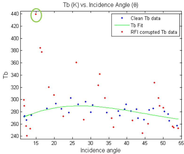
Fig. 5.6: (a) SMOS H-pol Tb snapshot with a clear RFI spot at 450K (bright red) (b) Angular domain representation of the same RFI pixel with flagged RFI Tbs (red), RFI-free Tbs (blue) and cubic fit (green). The circled sample in (b) is the same pixel as the red hot spot in (a)
