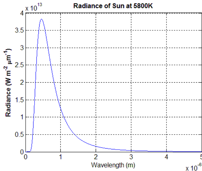
Fig. 1.1: Black-body radiance of the Sun at 5800K. The peak wavelength is around 450-500nm, which is in the middle of the visible spectrum.
