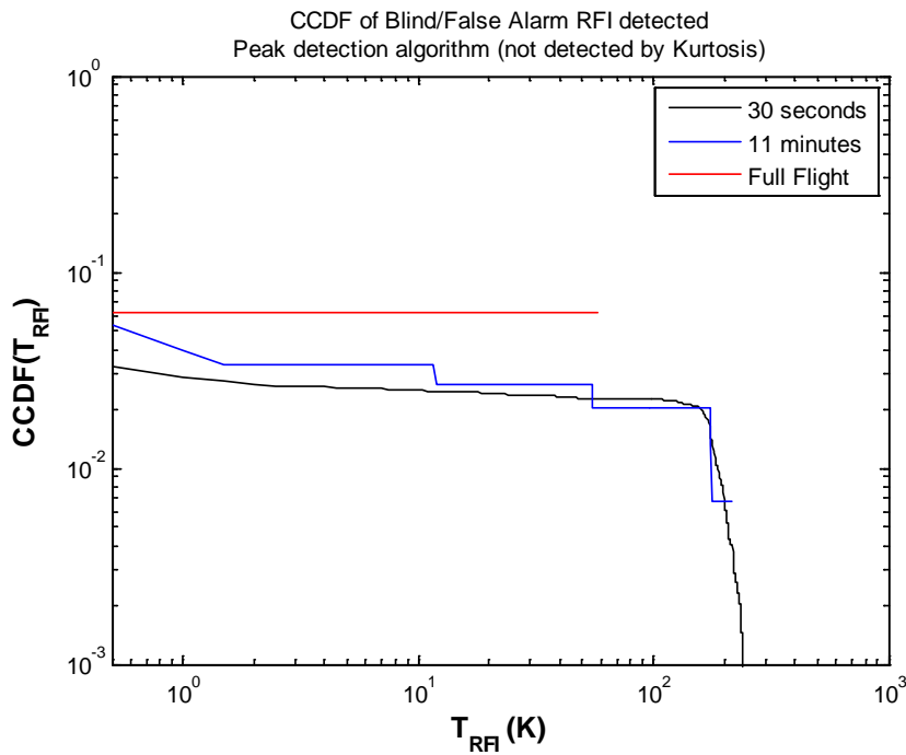
Fig. I.4: CCDF of brightness temperature contribution of blind RFI, i.e. RFI detected using the peak detection algorithm but not detected by Kurtosis
