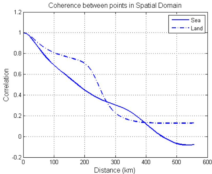
Fig. 5.5: Correlation statistics between a spatial domain sample and its neighboring pixels based on two SMOS half-orbits. The dashed line represents land statistics and solid line represents sea statistics.
