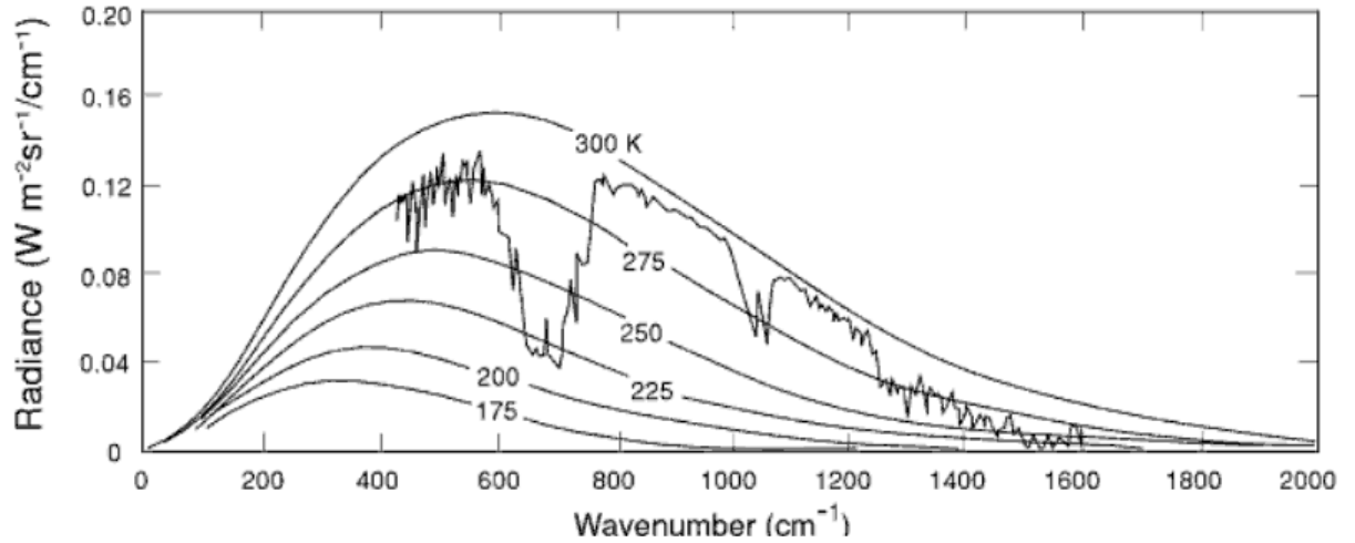
Fig. 1.4: Theoretical Planck radiance curves for a number of the earth's atmospheric temperatures as a function of wavenumber. Also shown is a thermal infrared emission spectrum observed from the Nimbus 4 satellite indicating radiance at the top of the atmosphere. (courtesy [4])
