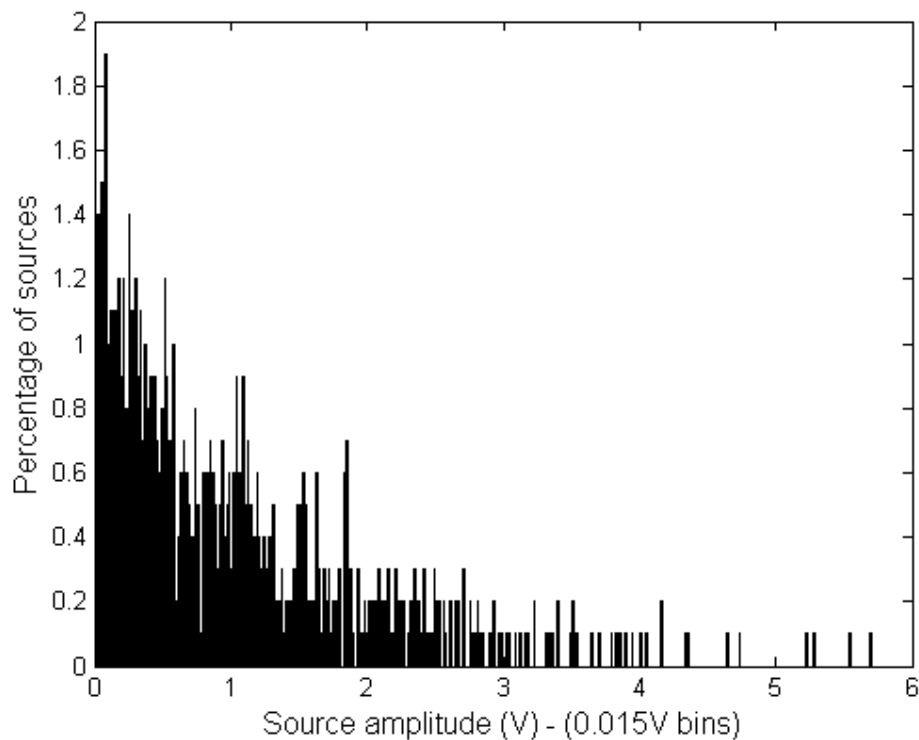
Fig. 4.2: Exponential pdf applied for amplitude of individual RFI sources, the mean of the exponential pdf is a scalable parameter based on required output power. The above plot has a mean of 1V.
