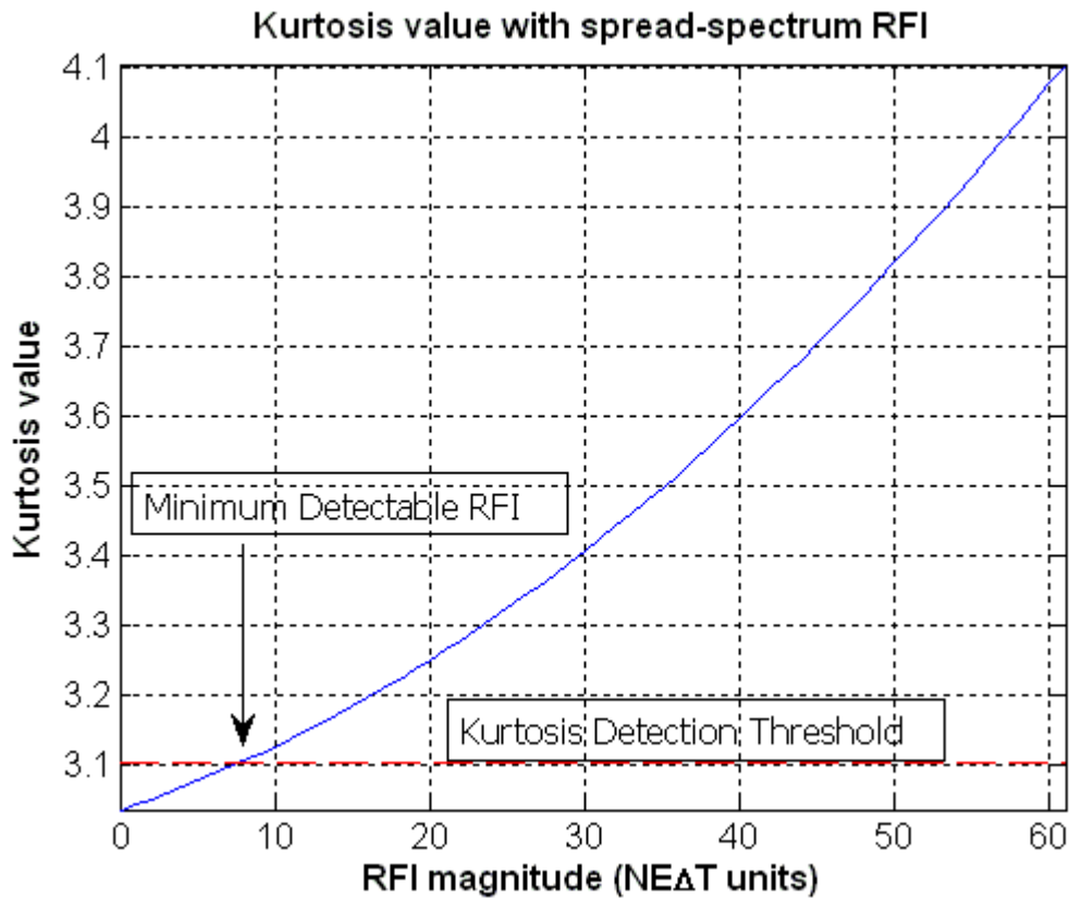
Fig. II.4: Plot indicating change in kurtosis as a function of the RFI magnitude for spread spectrum interference. The dashed line indicates the kurtosis 3\sigma detection threshold
