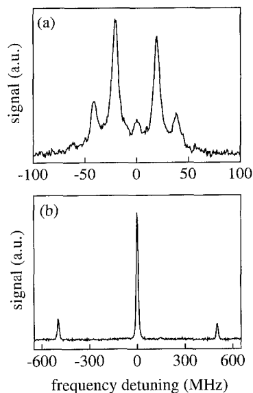
Fig. 4. Spectra of the laser output modulated at 20 MHz (a) and 500 MHz (b). The spectra are obtained by observing the transmission of a scanning Fabry-Pérot resonator (spectral resolution 10 MHz)). We have used -13 dBm RF-power in (a) and 15 dBm in (b) respectively.
