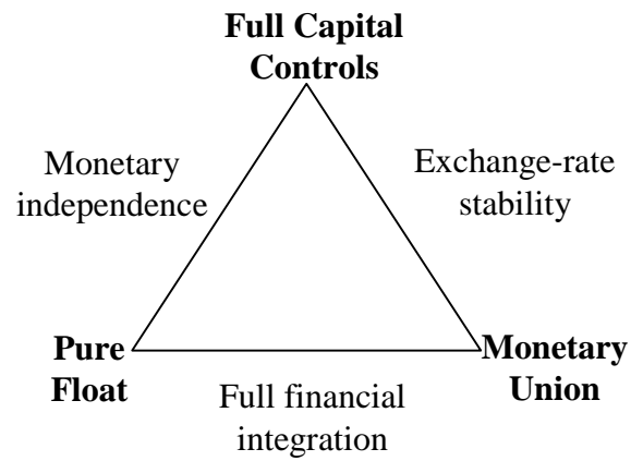
Figure 3: The Impossible Trinity
