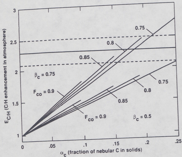
Figure 5-6. Predicted C/H ratio in the atmosphere of Jupiter (in units of the solar ratio) as a function of the fraction of the carbon of the outer solar nebula that was contained in solid bodies. The solid horizontal line shows the observed ratio and the dashed lines alternative values allowed by measurement uncertainties. The various slanting lines show predicted values for various choices of the fraction of nebular carbon in the form of CO, F_{CO} , and the fraction of planetesimals that dissolved in Jupiter's envelope during its formation, \beta_c .
