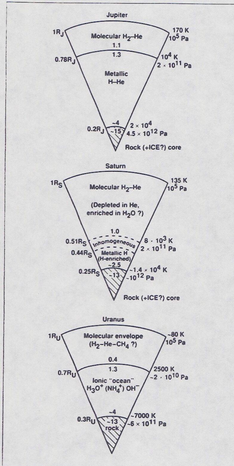
Figure 5-1. Schematic representation of the interior structure of the giant planets. Neptune has a structure similar to that of Uranus and so it is not shown. The numbers on the left show distance from the center in units of the planet's radius; the numbers on the right show pressure and temperature in units of pascals ( =10^{-5} bars) and degrees Kelvin, respectively; and the numbers in the center show density in units of that of liquid water.
