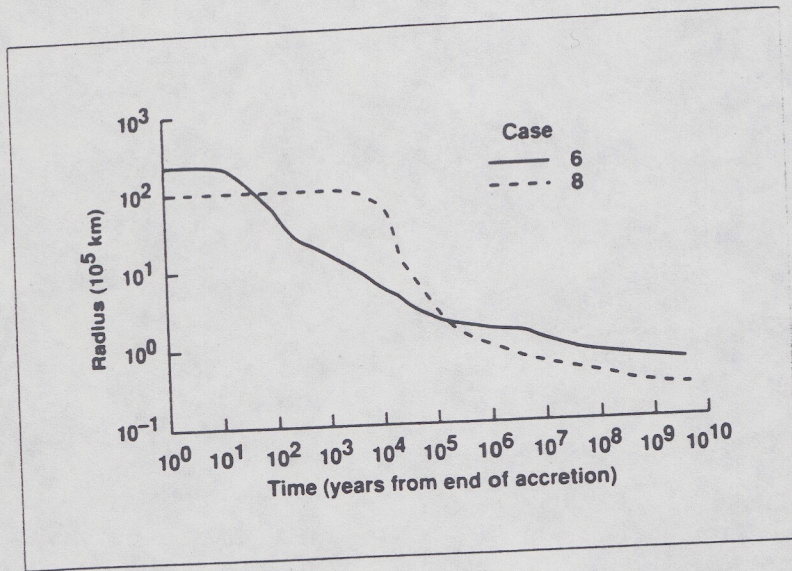
Figure 5-5. Radius of Saturn (solid) and Uranus (dashed) as a function of time from the completion of their accretion.
