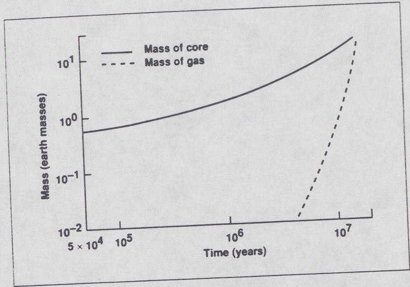
Figure 5-4. Envelope mass (dashed) and core mass (solid) as a function of time for a model of the growth of a giant planet for which the planetesimals were accreted at a constant rate of 10^{-6} Earth masses per year.
