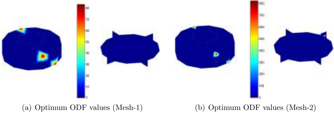
Figure 3.5: Optimum ODF representation for the thermal buckling problem
