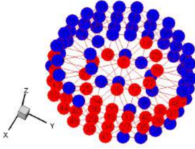
Figure 2.1: ODF representation in the Rodrigues fundamental region for hexagonal crystal symmetry showing the location of the k=50 independent nodes of the ODF in red color
