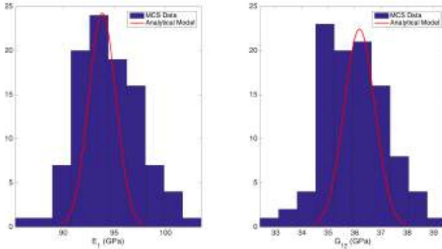
Figure 4.13: Probability histograms of E_1 and G_{12}
