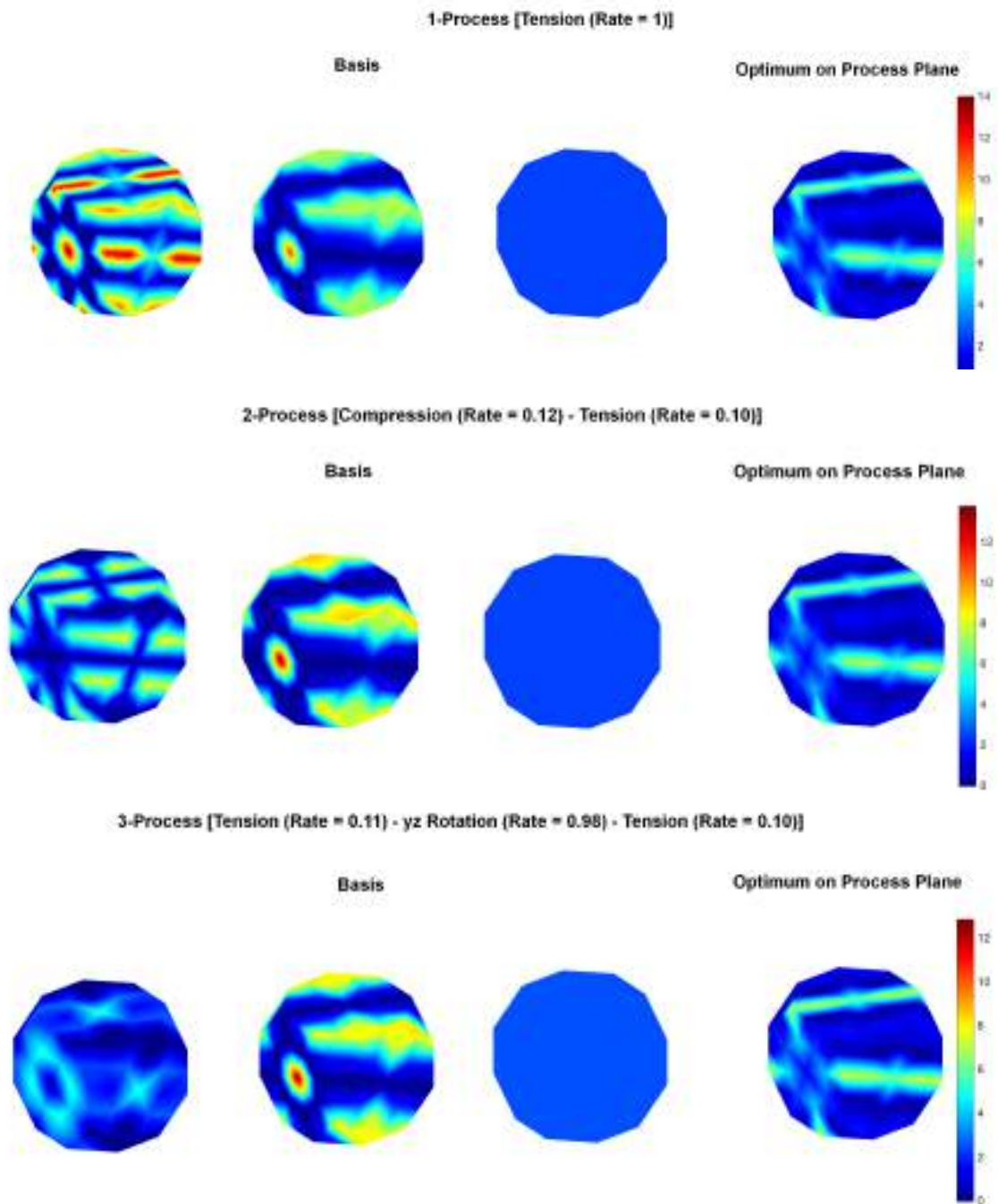
Figure 6.4: Optimum microstructures on process planes identified with ODF matching approach
