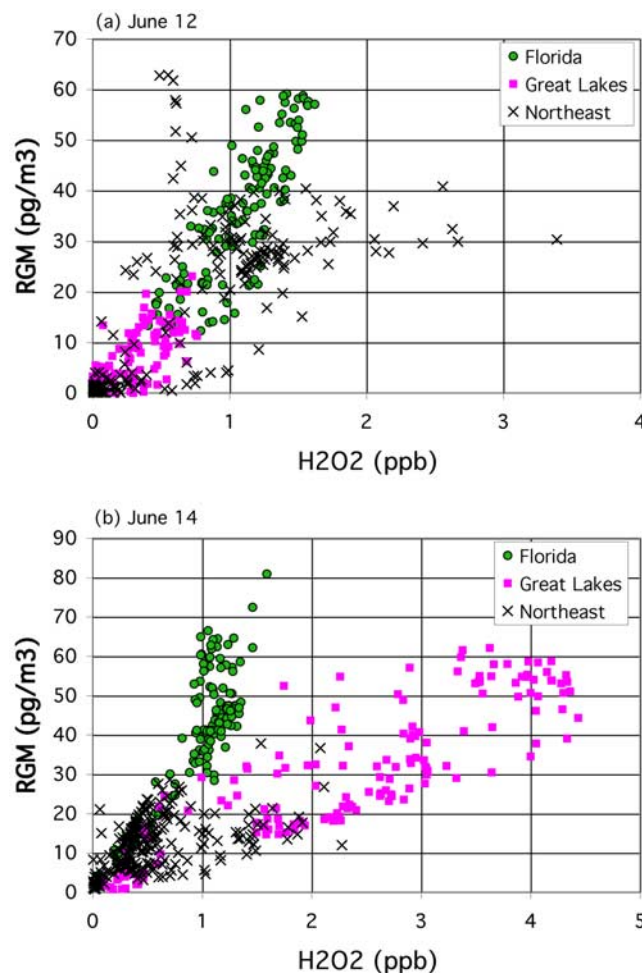
Figure 10. Model correlation between RGM ( \text{pg m}^{-3} ) and \text{H}_2\text{O}_2 (ppb) for the south Florida (green circles), northeast (crosses) and Great Lakes (pink squares) subregions identified in Figure 1. Correlations are for (a) 12 June and (b) 14 June, both at 0–0.2 km altitude and 1700 LT.
