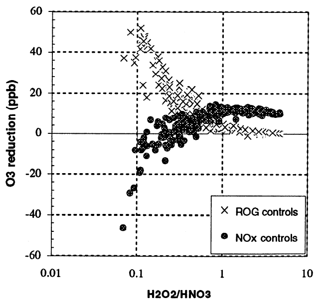
Figure 5. Predicted reduction in peak O_3 (ppb) resulting from a 35% reduction in the emission rate for anthropogenic ROG (crosses) and from a 35% reduction in the emission rate for \text{NO}_x (solid circles), plotted against \text{H}_2\text{O}_2/\text{HNO}_3 coincident with the ozone peak in the simulation for the Lake Michigan base case scenario.
