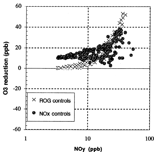
Figure 1b. Predicted reduction in peak O_3 (ppb) resulting from a 35% reduction in the emission rate for anthropogenic ROG (crosses) and from a 35% reduction in the emission rate for NO_x (circles), plotted against NO_y (ppb) coincident with the ozone peak in the simulation for the Lake Michigan scenario with doubled anthropogenic ROG [from Milford et al. , 1994].
