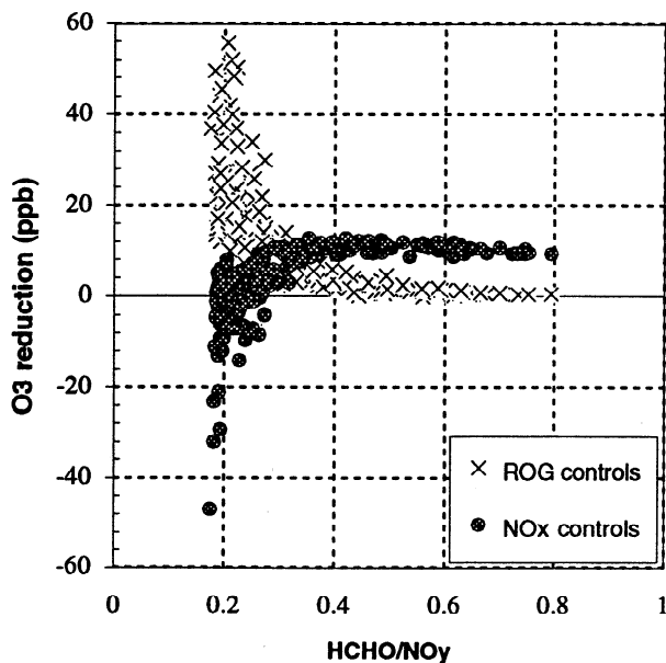
Figure 4. Predicted reduction in peak O_3 (ppb) resulting from a 35% reduction in the emission rate for anthropogenic ROG (crosses) and from a 35% reduction in the emission rate for \text{NO}_x (solid circles), plotted against \text{HCHO}/\text{NO}_y coincident with the ozone peak in the simulation for the Lake Michigan base case scenario.
