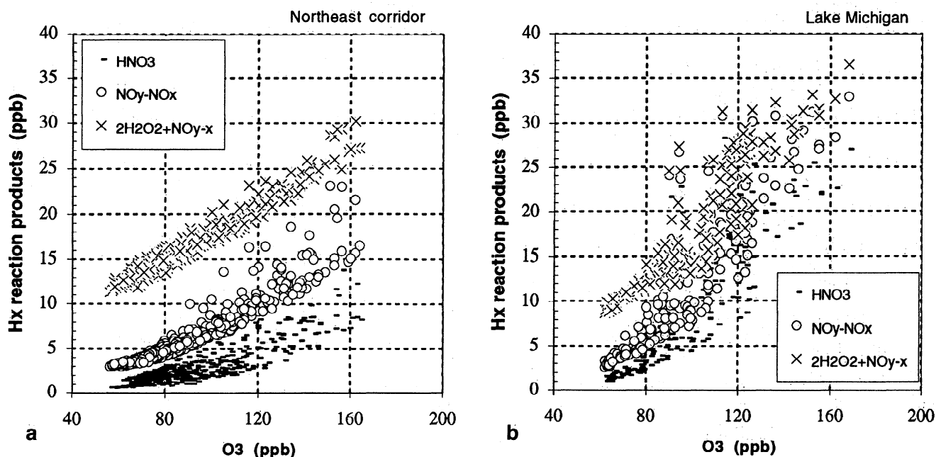
Figure 10. \text{HNO}_3 (points), \text{NO}_y - \text{NO}_x (circles) and \text{H}_2\text{O}_2 + (\text{NO}_y - \text{NO}_x) (crosses) versus \text{O}_3 , all in ppb at 1800 LT in simulations for (a) the northeast corridor and (b) the Lake Michigan airshed.
