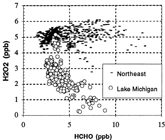
Figure 8. \text{H}_2\text{O}_2 versus HCHO (ppb) at 1800 LT in simulations for the northeast corridor (points) and the Lake Michigan airshed (circles).
