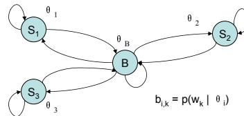
Figure 4: A 3-theme HMM
