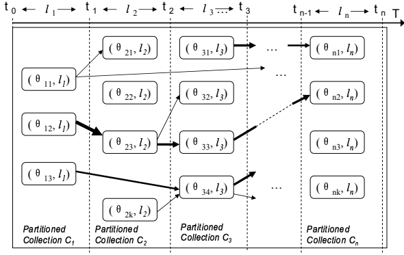
Figure 3: An example of a theme evolution graph
