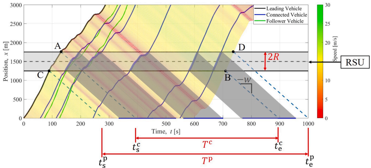
Fig. 2. Illustration of the traffic flow on a highway where the measured lead vehicle trajectory is black, measured follower vehicle trajectories are green, the trajectories of simulated vehicles are colored according to their speeds, and connected vehicles are highlighted by blue. A single RSU is located along the road with communication range R as indicated and it provides traffic predictions for location x = 0 . The duration of the potential coverage zone is indicated by T^p = t_e^p - t_s^p , and the duration of the constant coverage zone is indicated by T^c = t_e^c - t_s^c . The time intervals covered by predictions are shown by the blue sections. (For interpretation of the references to color in this figure legend, the reader is referred to the web version of this article.)
