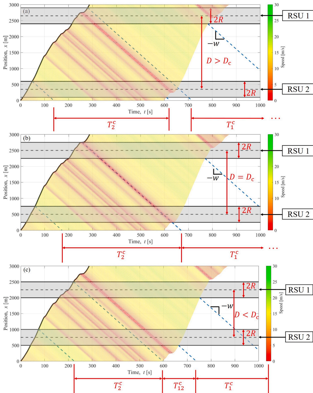
Fig. 7. Setup with two RSUs where the distance of the RSUs is (a) larger than the critical distance D > D_c , (b) equal to the critical distance D = D_c and (c) smaller than the critical distance D < D_c .
