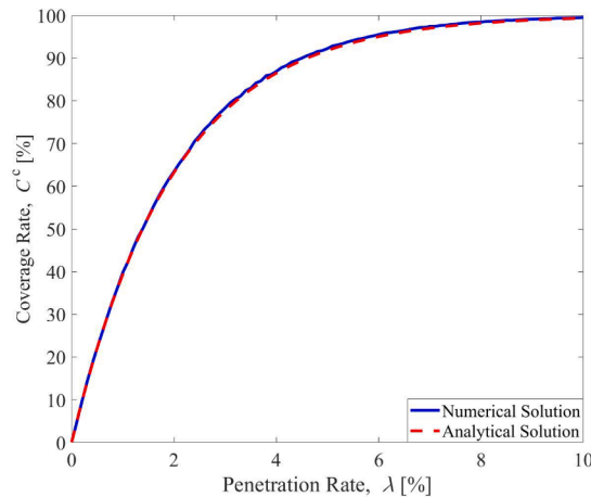
Fig. 4. Numerical and analytical results for the constant coverage rate as a function of the penetration rate for a single RSU with communication range R = 250 m.
