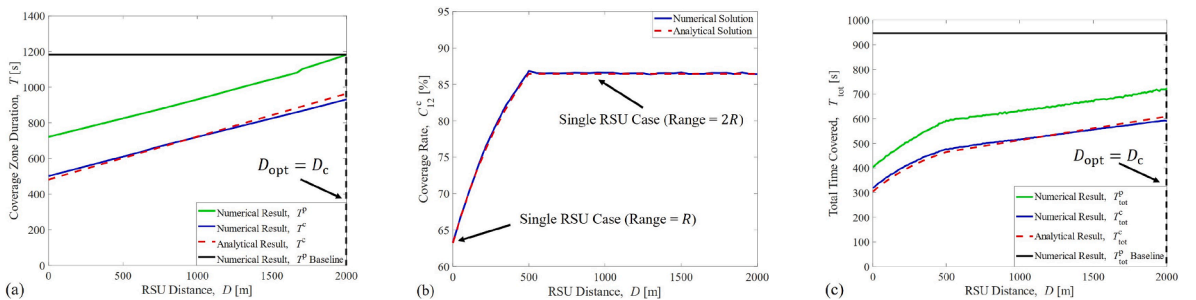
Fig. 8. (a) The duration of the potential and constant coverage zones for two RSUs as a function of their distance. (b) Coverage rate C_{12}^c as a function of RSU distance. (c) The total time covered by two RSUs as a function of their distance. The parameters are R = 250 m and \lambda = 2\% . The mean position of the two RSUs is fixed to the location x = 1500 m. The exact numerical results of T^p and T_{tot}^c given by (6) and (10) are compared to the approximate analytical results obtained by variants of (7) and (23) that use constant speed approximation (with v = 11 m/s). The exact numerical results for the baseline are also shown for comparison.
