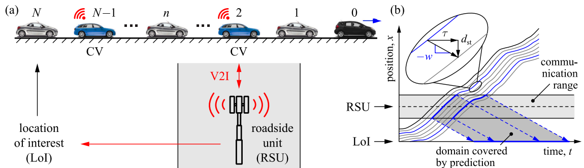
Fig. 1. (a) Traffic flow consisting of non-connected (gray) and connected vehicles (blue), where a roadside unit provides traffic prediction for a location of interest. (b) Illustration of the vehicle trajectories, the RSU's communication range, and the region where traffic prediction is possible. (For interpretation of the references to color in this figure legend, the reader is referred to the web version of this article.)
