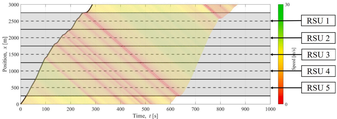
Fig. 6. Baseline scenario for multiple RSU deployment where five RSUs are located such that any point along a road segment lies within the communication range of one of the RSUs.
