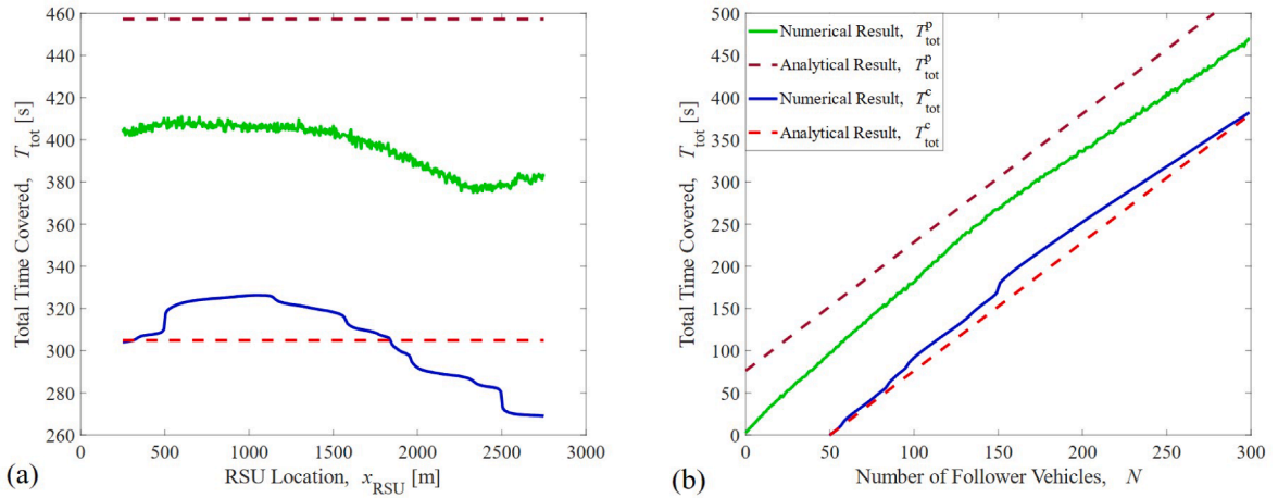
Fig. 5. The total time covered for the potential and constant coverage zones as function of (a) the RSU location x_{RSU} (when N = 250 ) and (b) the number N of follower vehicles (when x_{RSU} = 1500 m) for the setup illustrated in Fig. 2. The CV penetration rate is set to \lambda = 2\% . Both panels compare the exact numerical results given by (12) and (13) to the approximate analytical results obtained from (15) that uses constant speed approximation (with v = 11 m/s).
