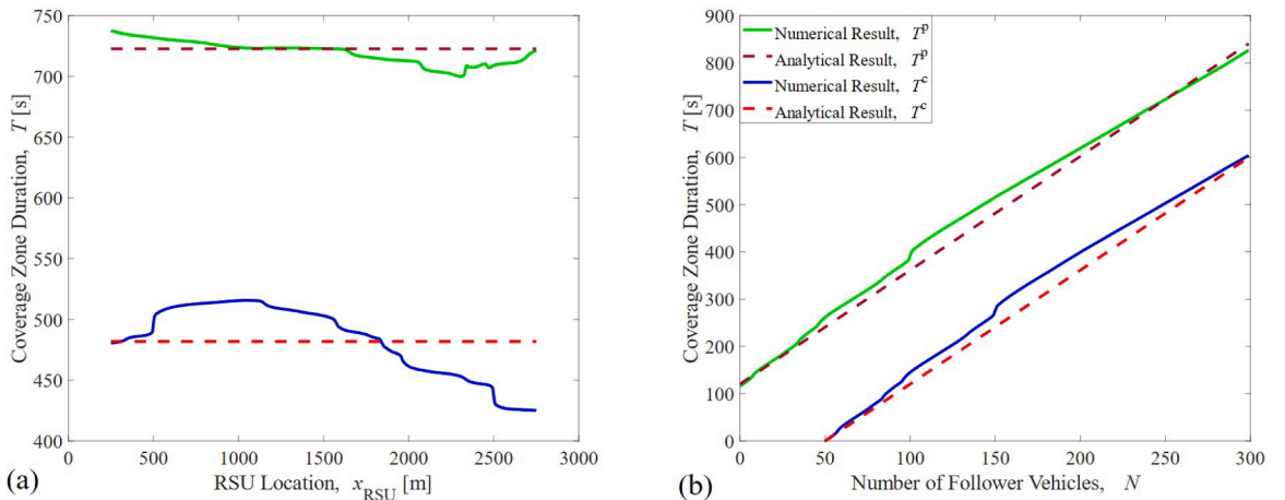
Fig. 3. The duration of the potential and constant coverage zones as function of (a) the RSU location x_{RSU} (when N = 250 ) and (b) the number N of follower vehicles (when x_{RSU} = 1500 m) for the setup illustrated in Fig. 2. Both panels compare the exact numerical results given by (6) and (8) to the approximate analytical results obtained from (7) and (9) that use constant speed approximation (with v = 11 m/s).
