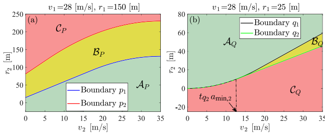
Fig. 2. Boundaries in the (v_2, r_2) plane for given v_1, r_1 values as indicated. (a) Boundaries p_1 and p_2 separating sets \mathcal{A}_P, \mathcal{B}_P, and \mathcal{C}_P . (b) Boundaries q_1 and q_2 separating sets \mathcal{A}_Q, \mathcal{B}_Q, and \mathcal{C}_Q .
