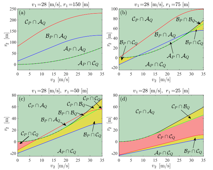
Fig. 3. Conflict charts for given v_1, r_1 values, where each region is an intersection of sets \mathcal{A}_P, \mathcal{B}_P, and \mathcal{C}_P and sets \mathcal{A}_Q, \mathcal{B}_Q, and \mathcal{C}_Q .
