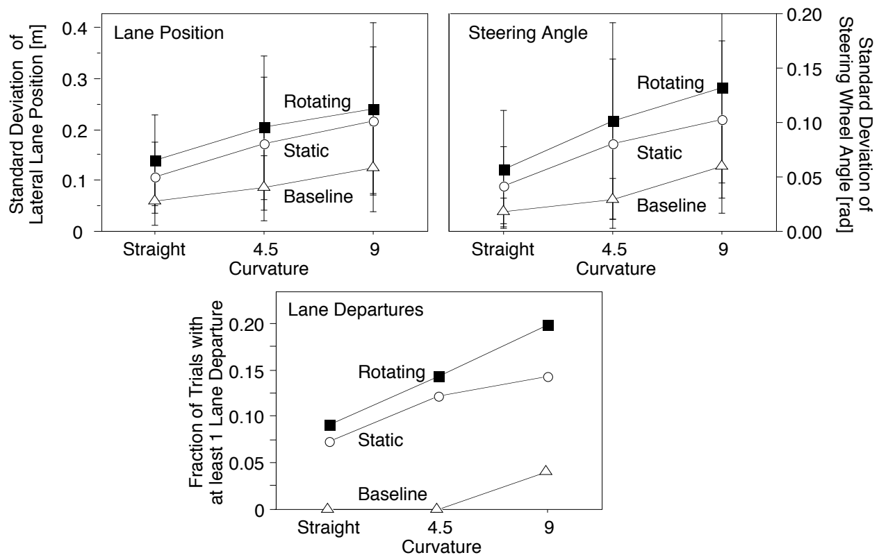
Figure 7. The effect of curvature and task on lateral vehicle control
