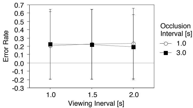
Figure 9. The effect of viewing and occlusion intervals on error rate
