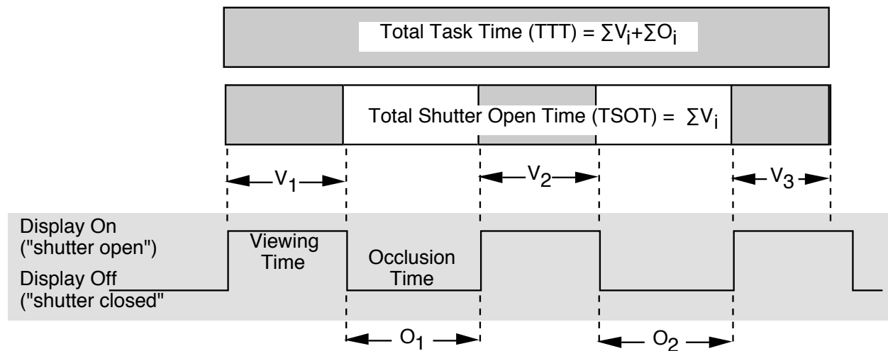
Figure 16. Diagram of timing measures
