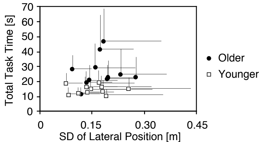
Figure 18. The tradeoff between total task time and standard deviation of lane control (Each point and line represent mean and 1 SD of one subject's trials)
