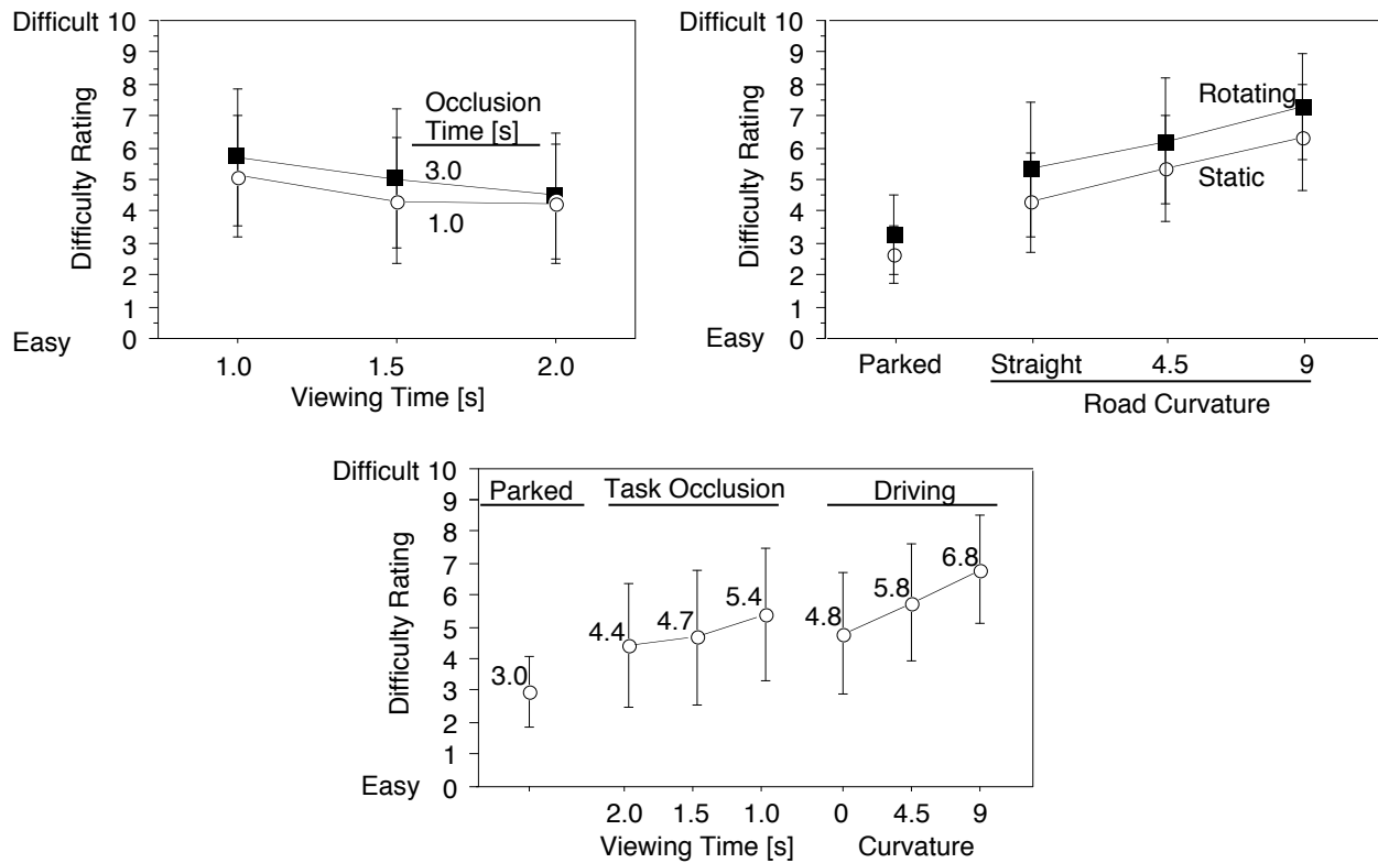
Figure 19. Subjective difficulty ratings of task occlusion (top left), driving (top right), and a side-by-side comparison (bottom)
