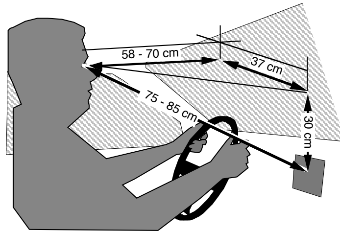
Figure 2. The location of the in-vehicle displays
