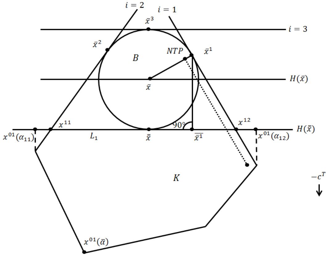
Figure 3: The Ball B with center \bar{x} , the largest ball inside K with this center, has 3 touching facets numbered i = 1, 2, 3 with touching points \bar{x}^1, \bar{x}^2, \bar{x}^3 respectively. The dotted line beginning with the NTP corresponding to i = 1 , is the descent step D5.1 from it, and the point at the other end of this line is the output point from this step. For descent steps D5.7, The objective plane H(\bar{x}) is moved parallel to itself in the direction -c^T until it becomes a tangent plane to B with its touching point \bar{x} . Corresponding to i = 1 , \bar{x}^1 is the orthogonal projection
