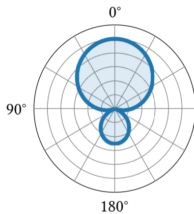
Hypercardioid
