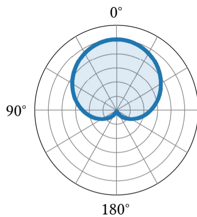
Cardioid
