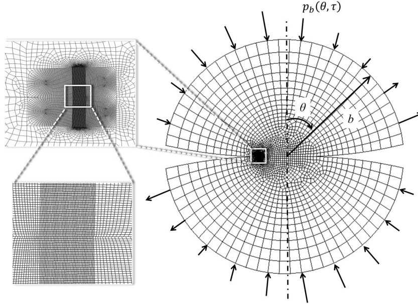
Figure 4: Finite-element model.
