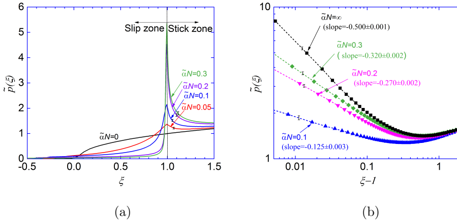
Figure 6: (a) Evolution of the dimensionless contact pressure \tilde{p}(\xi) with the normalized number of loading cycles \tilde{\alpha}N , from elastic analysis. (b) Plots showing how the stress field near the stick-slip boundary evolves to a crack-like inverse-root singularity as wear progresses. \xi - 1 represents the normalized distance from the edge of the wear scar.
