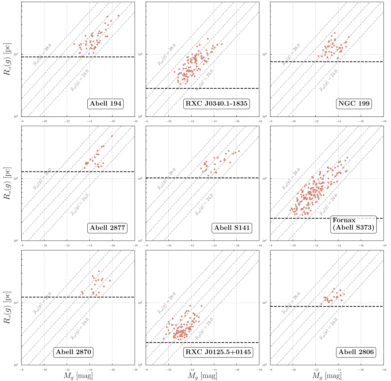
Figure 14. Size–luminosity relation for LSBGs around the associations of the most prominent overdensity peaks, presented in Table 2. We have assumed that all LSBGs within an angle corresponding to a physical radius of 0.5 Mpc at the distance of the association belong to it. With the dashed horizontal lines, we show the physical scale corresponding to the radius cut r_{1/2}(g) > 2''.5 at the distance of the cluster. We also show (dashed, diagonal gray lines) the lines of constant mean surface brightness.
