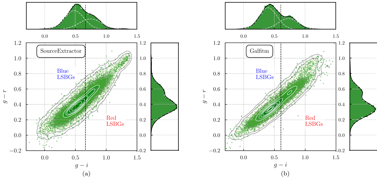
Figure 5. Color-color diagram of our LSBG sample, using (a) SourceExtractor MAG_AUTO parameters and (b) magnitudes derived by fitting with galfitm . In both cases, we observe a bimodality in the g-i and g-r color distributions. We separate the total sample into red and blue galaxies, based on their g-i color value: we fit the g-i distribution with a Gaussian mixture model with two Gaussians (gray dashed lines in the top panels) and find the intersection point. This is at g-i = 0.66 and g-i = 0.60 for the SourceExtractor and galfitm cases, respectively (black vertical dashed lines). We use the intersection point derived from the galfitm distribution to define red and blue LSBG samples.
