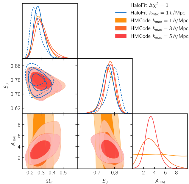
Figure 13. Constraints on cosmological and baryonic feedback parameters from DES Y3 cosmic shear power spectra. In blue, we show constraints for the fiducial model, i.e. using HALOFIT. In orange to red, we show constraints using HMCODE with one free parameter, while varying the k_{\max} cut-off from 1 to 5 h \text{ Mpc}^{-1} (see Fig. 4). We also show, with dashed lines, the constraints for the fiducial HALOFIT model and the k_{\max} = 1 h \text{ Mpc}^{-1} cut, which is even more conservative than our fiducial \Delta\chi^2 = 1 cut. Note that all constraints shown here use TATT to model intrinsic alignments and none include shear ratio information.
