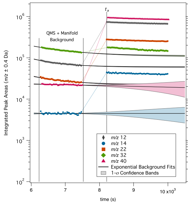
Figure 3. Integrated peak areas (cps * 0.8 Da-width peak) for the preferred ions of CO 2 ( m/z 22), Ar ( m/z 40), N 2 ( m/z 14), O 2 ( m/z 32), and CO ( m/z 12, with contributions from CO 2 ) are plotted against time for a typical SAM atmospheric experiment. TID 25217 is shown here; see Table 1 for details. The background measurement (no atmospheric gas ingested into the QMS) is accomplished in the experiment time between 6,278 and 7,468 s. Mars atmosphere is then ingested and measured by the mass spectrometer between 8,211 and 10,000 s. To perform the background correction, the exponential decay in the residual gas background signal shown in the bracketed region is fit and extrapolated to the time of the first fractional atmospheric scan at time t_a . The fit value at t_a is then used to estimate the contribution of the background to the signal during the sample ingest. As can be seen in this example, only the m/z 32 background is >10% of the atmospheric signal. Confidence bands show the fit uncertainties used to estimate the error in the background correction.
