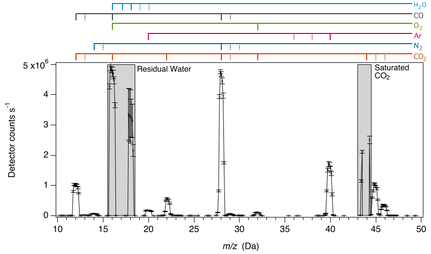
Figure 2. A typical atmospheric mass spectrum taken in fractional scan mode with the residual background signal subtracted. TID 25217 is shown here; see Table 1 for details. The error bars show the standard deviation of the average counts per second (cps) from multiple scans over a \sim 7 -minute period. The gray bars indicate regions of the spectrum which are not used for VMR calculations, either due to decreasing residual water signal or high counts from the primary \text{CO}_2 ion ( m/z 44) that saturate the detector. Integrated peak areas used for quantitative determination of the volume mixing ratios are determined from a \pm 0.4 Da window around each nominal m/z .
