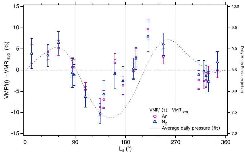
Figure 11. The global annual mean values of Ar and N 2 (Figure S5) were subtracted from the pressure-corrected mixing ratios of Ar and N 2 (VMR', equation (5)) at each seasonal point and plotted as a percent deviation from the average. In this way, the observed seasonal cycle of Ar and N 2 can be compared directly to a flat annual mean that removes the mixing ratio changes introduced by fluctuating CO 2 pressures. If there were no influence of transport, the corrected VMR' values would appear on the dashed zero line. The polynomial fit to the daily mean pressure data is shown as a gray dashed line for comparison to the annual pressure cycle.
