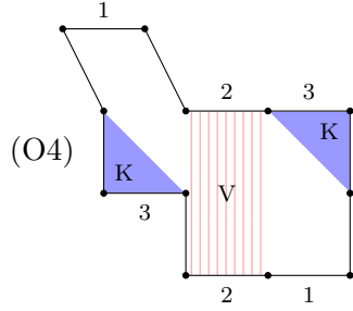
FIGURE 6.3. In the proof of Lemma 6.5, eventually there is a vertical cylinder V shaded with vertical lines above, and a cylinder K shaded solid above.
